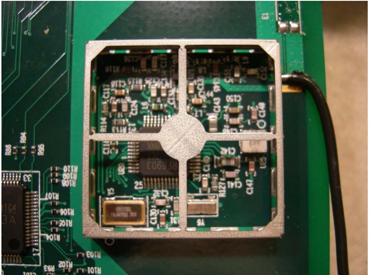
Figure 2: PCB Front without Shields – Shielded area only
