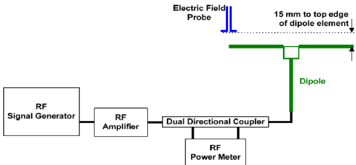
Fig.4 System verification
