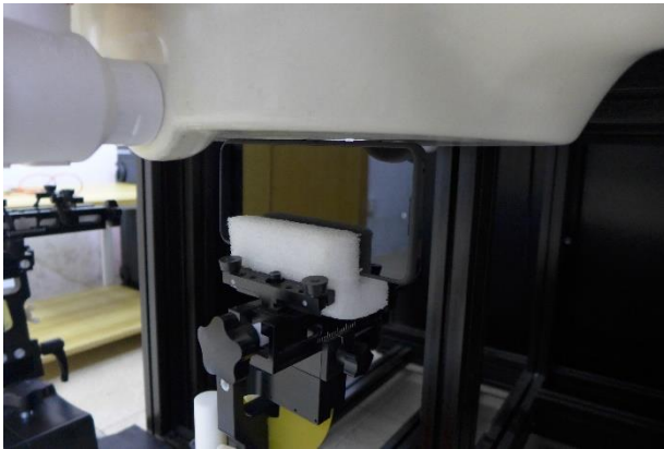
Photo 18: Top side 0mm
