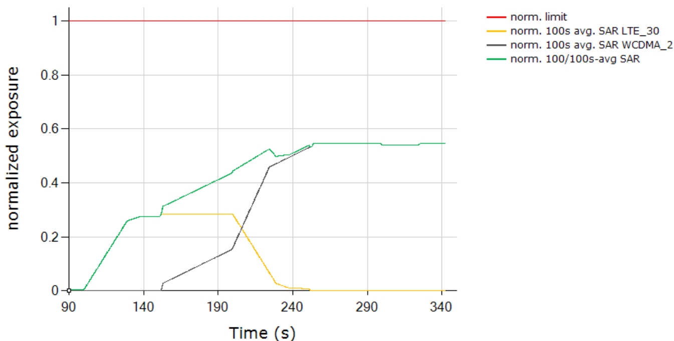
Total Normalized Time-averaged RF Exposure Tech: LTE, Band 30 / Tech: WCDMA, Band 2
