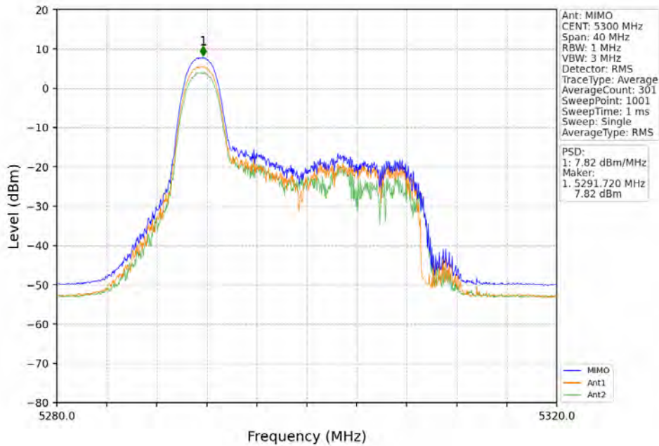
802.11ax(HEW20)_MCH_5300MHz_RU26_Left_MIMO_NTNV
