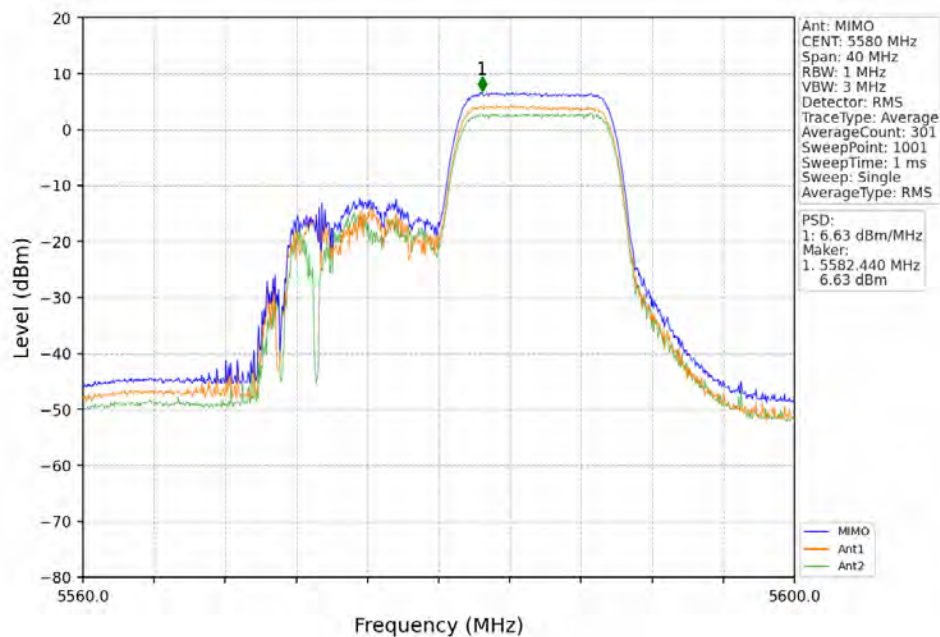
802.11ax(HEW20)_MCH_5580MHz_RU106_Right_MIMO_NTNV
