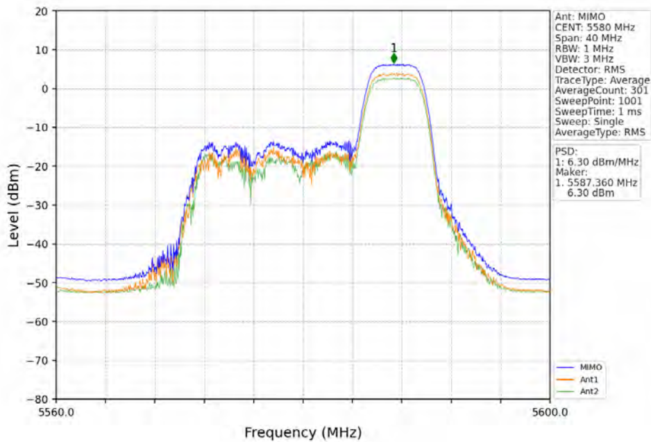
802.11ax(HEW20)_MCH_5580MHz_RU52_Right_MIMO_NTNV
