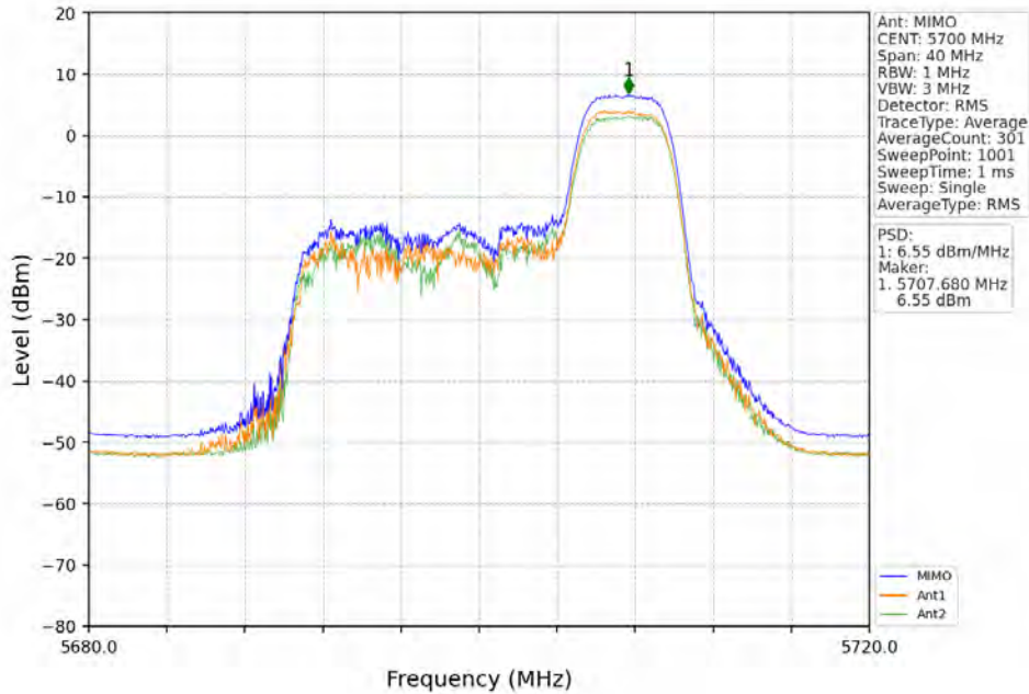
802.11ax(HEW20)_HCH_5700MHz_RU106_Left_MIMO_NTNV
