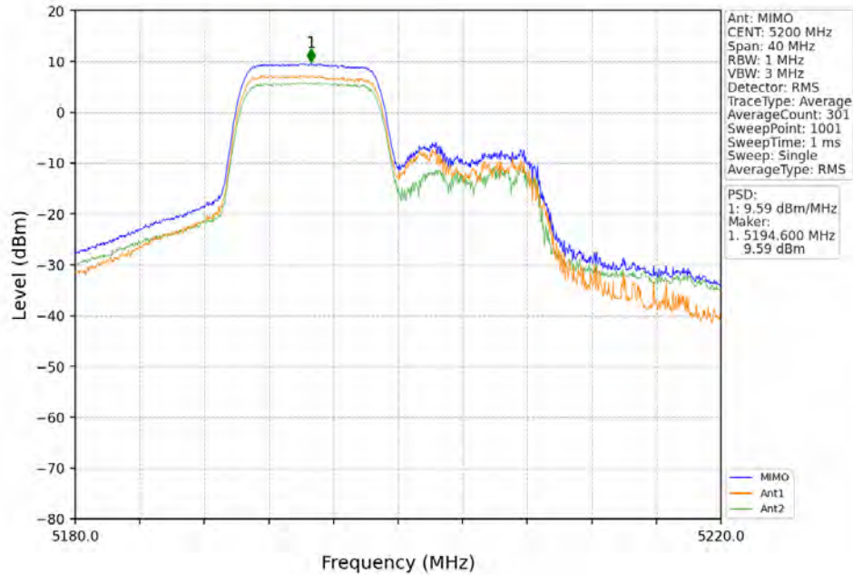
802.11ax(HEW20)_MCH_5200MHz_RU106_Right_MIMO_NTNV
