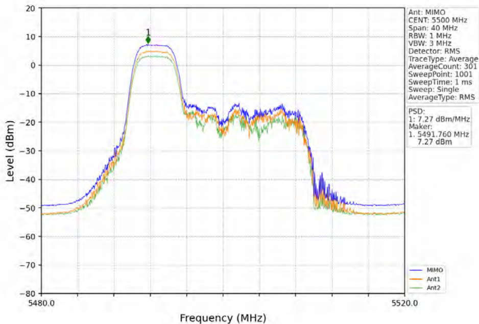
802.11ax(HEW20)_LCH_5500MHz_RU52_Left_MIMO_NTNV
