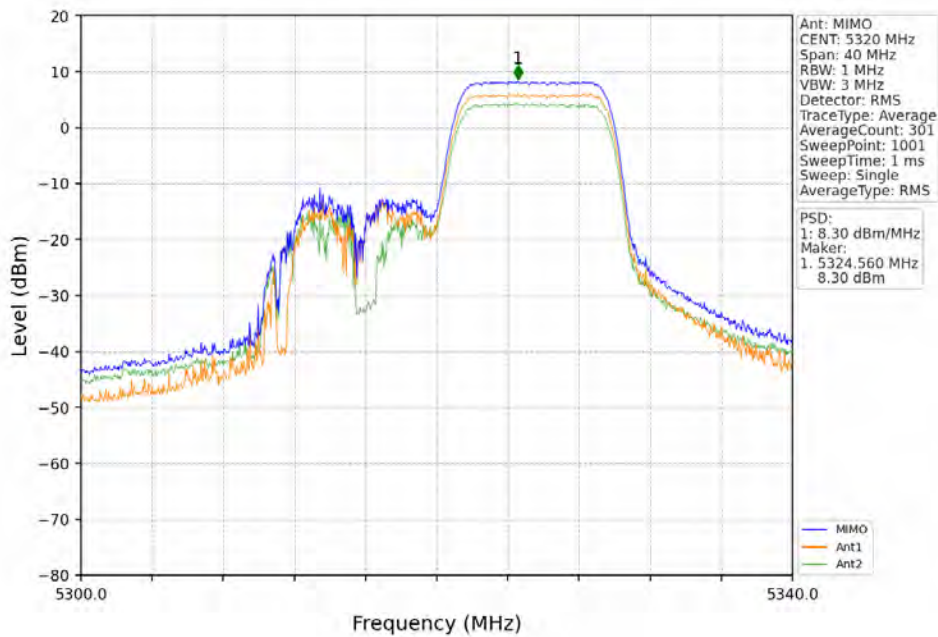
802.11ax(HEW20)_HCH_5320MHz_RU106_Right_MIMO_NTNV
