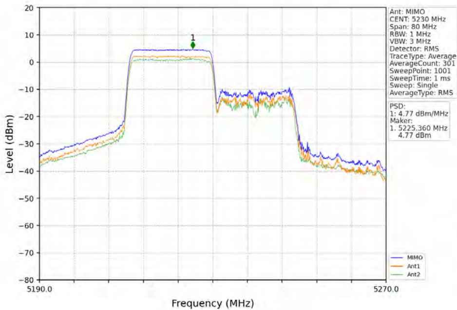
802.11ax(HEW40)_HCH_5230MHz_RU242_Left_MIMO_NTNV
