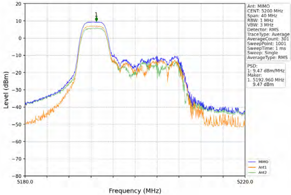
802.11ax(HEW20)_MCH_5200MHz_RU52_Right_MIMO_NTNV
