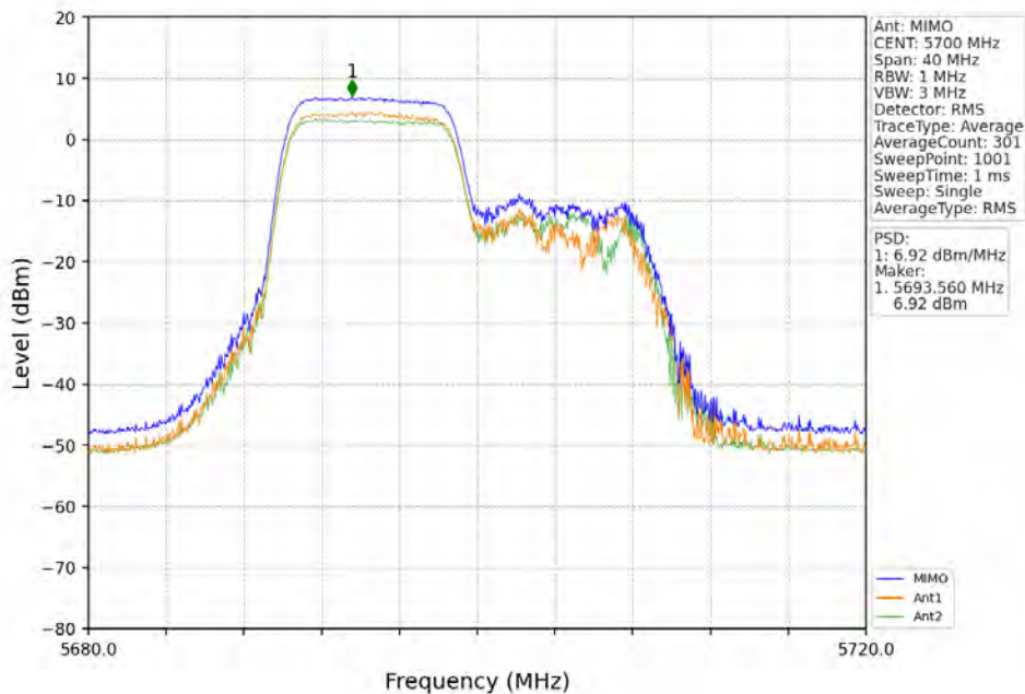
802.11ax(HEW20)_HCH_5700MHz_RU106_Left_MIMO_NTNV
