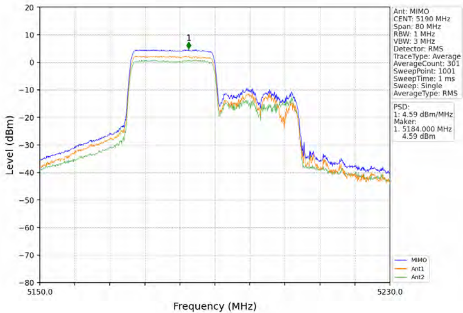
802.11ax(HEW40)_LCH_5190MHz_RU242_Right_MIMO_NTNV
