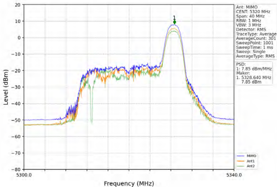
802.11ax(HEW20)_HCH_5320MHz_RU26_Right_MIMO_NTNV
