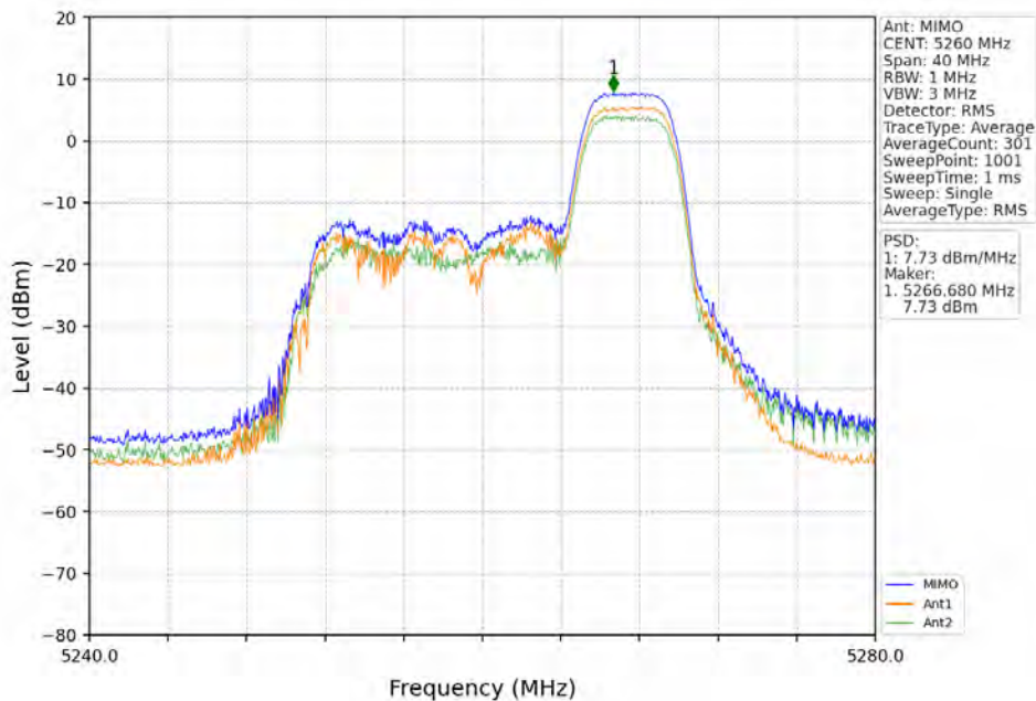
802.11ax(HEW20)_LCH_5260MHz_RU52_Right_MIMO_NTNV
