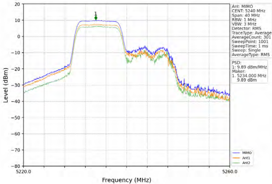
802.11ax(HEW20)_HCH_5240MHz_RU106_Left_MIMO_NTNV
