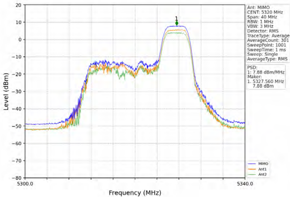
802.11ax(HEW20)_HCH_5320MHz_RU52_Right_MIMO_NTNV
