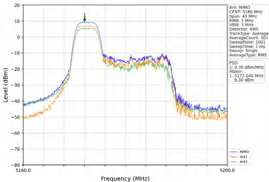
802.11ax(HEW20)_LCH_5180MHz_RU52_Left_MIMO_NTNV
