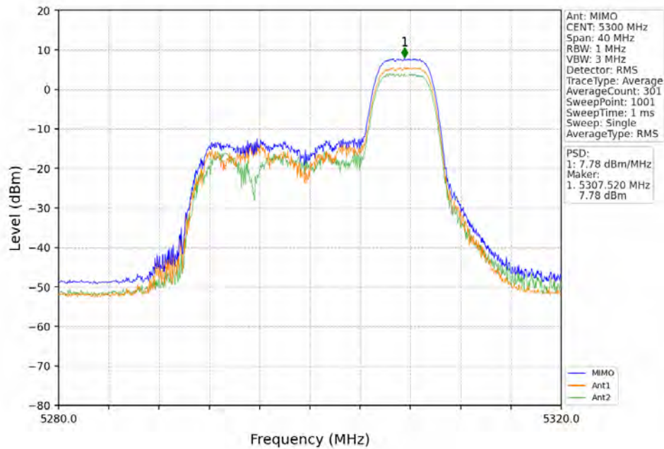
802.11ax(HEW20)_MCH_5300MHz_RU106_Left_MIMO_NTNV
