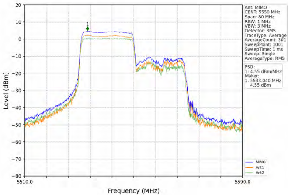
802.11ax(HEW40)_MCH_5550MHz_RU242_Left_MIMO_NTNV
