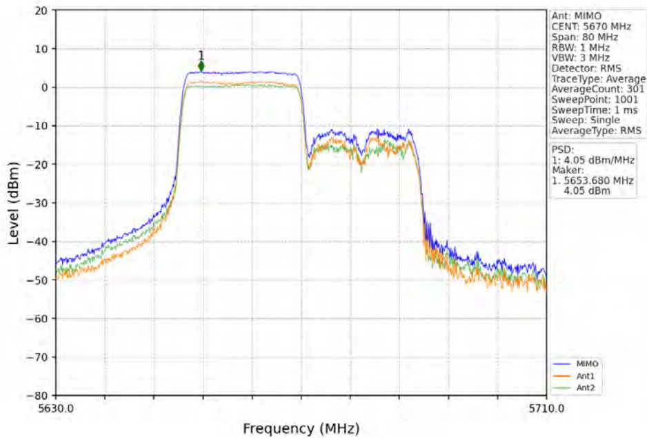
802.11ax(HEW40)_HCH_5670MHz_RU242_Right_MIMO_NTNV
