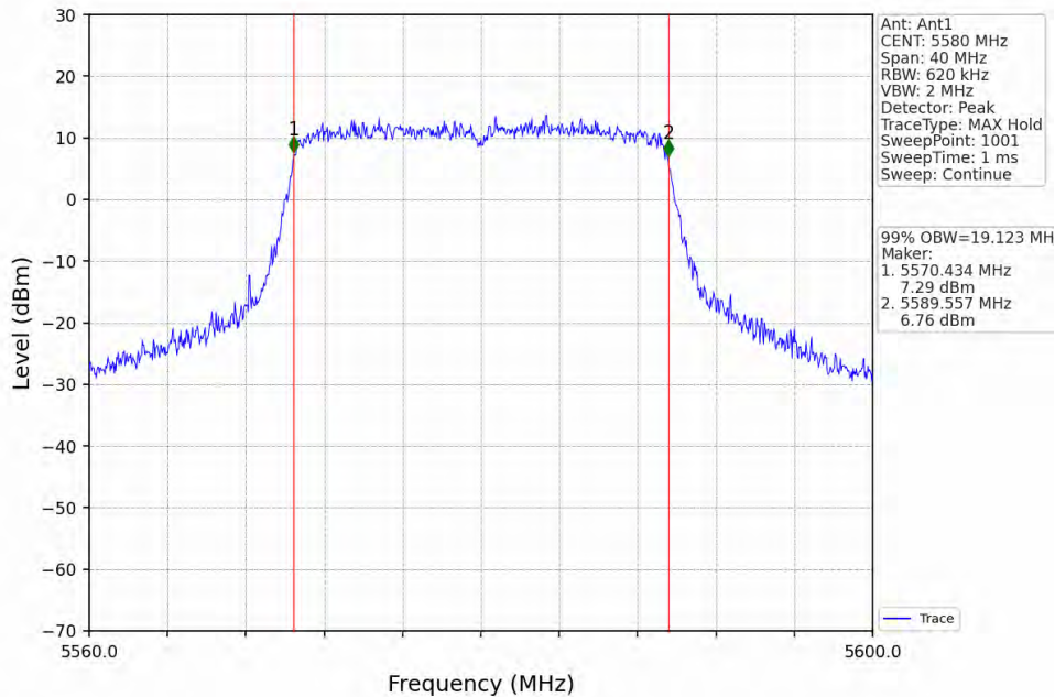
802.11ax(HEW20)_MCH_5580MHz_RU242_Left_Ant1_NTNV
