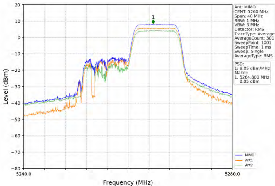
802.11ax(HEW20)_LCH_5260MHz_RU106_Right_MIMO_NTNV
