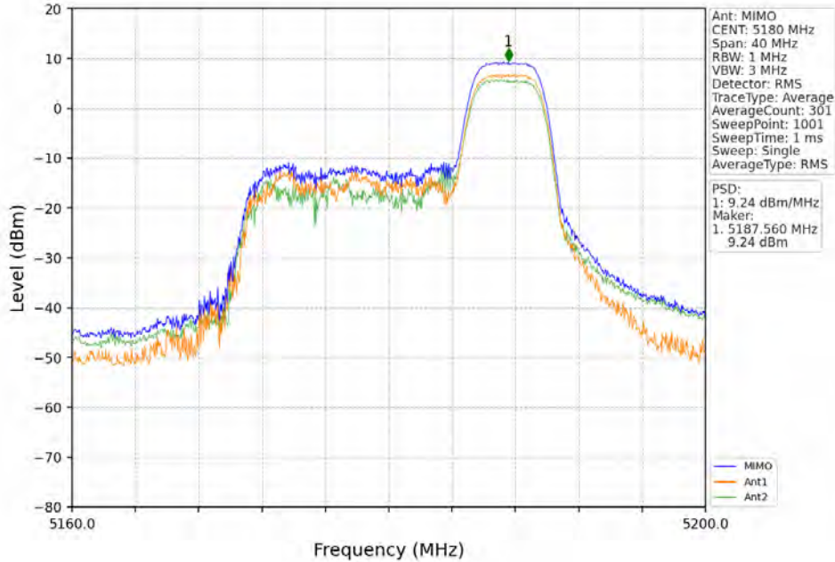
802.11ax(HEW20)_LCH_5180MHz_RU106_Left_MIMO_NTNV
