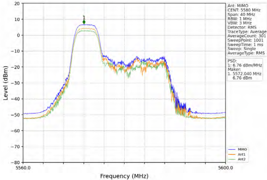
802.11ax(HEW20)_MCH_5580MHz_RU52_Right_MIMO_NTNV
