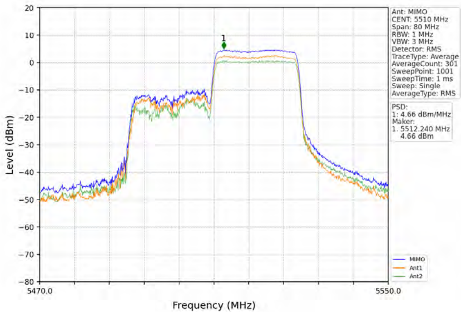
802.11ax(HEW40)_LCH_5510MHz_RU242_Right_MIMO_NTNV
