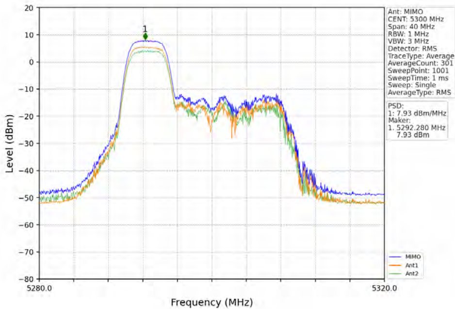
802.11ax(HEW20)_MCH_5300MHz_RU52_Left_MIMO_NTNV
