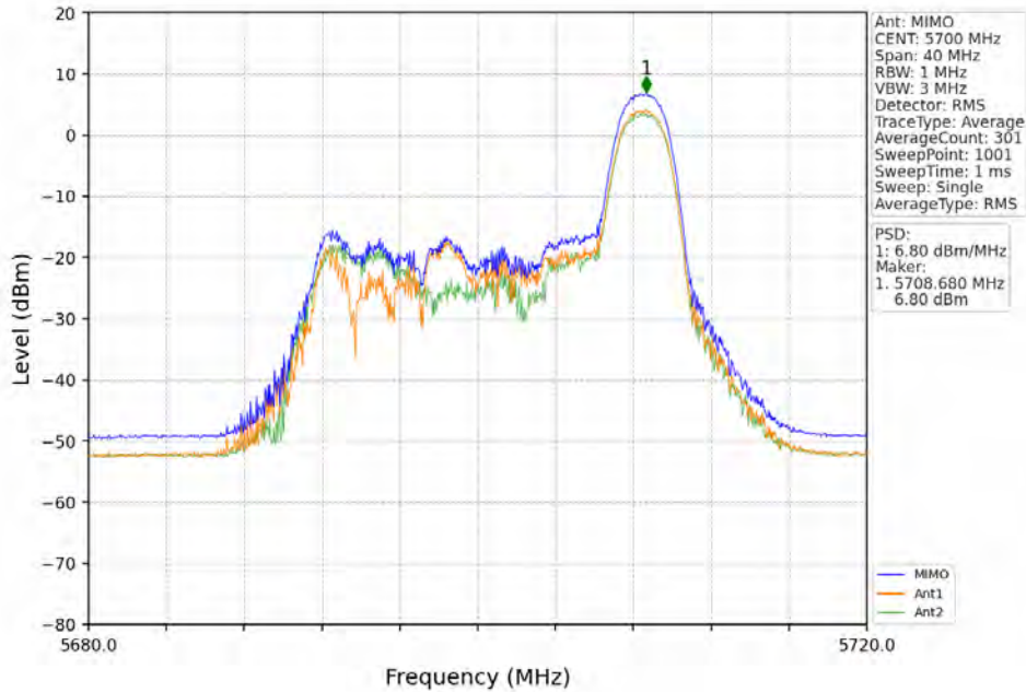
802.11ax(HEW20)_HCH_5700MHz_RU52_Left_MIMO_NTNV
