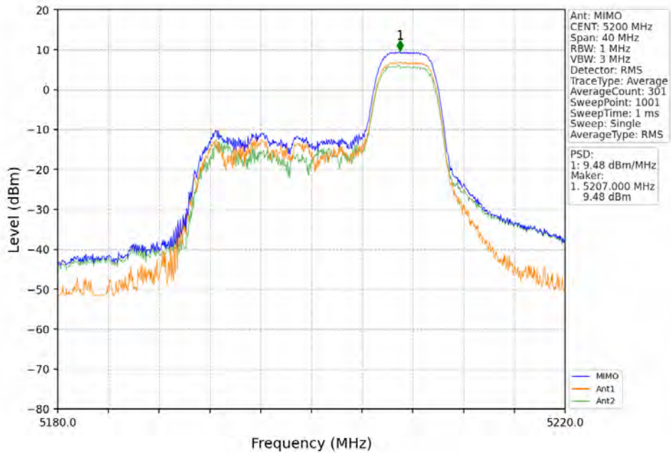
802.11ax(HEW20)_MCH_5200MHz_RU52_Right_MIMO_NTNV
