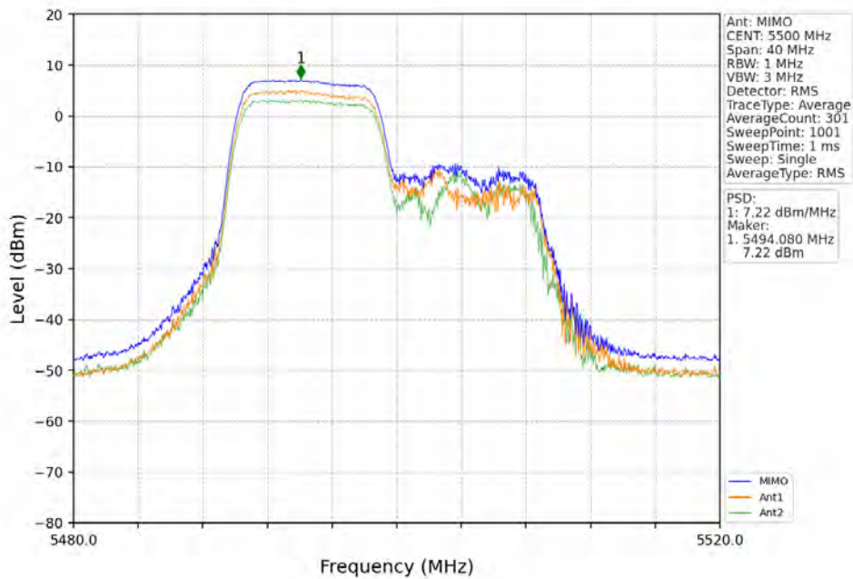
802.11ax(HEW20)_LCH_5500MHz_RU106_Left_MIMO_NTNV
