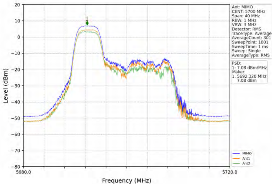
802.11ax(HEW20)_HCH_5700MHz_RU52_Left_MIMO_NTNV
