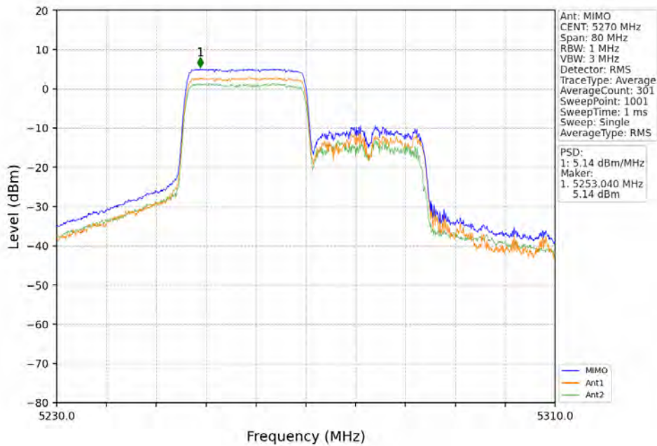
802.11ax(HEW40)_LCH_5270MHz_RU242_Right_MIMO_NTNV
