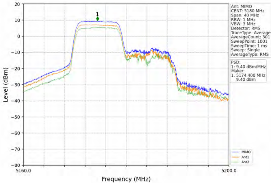
802.11ax(HEW20)_LCH_5180MHz_RU106_Left_MIMO_NTNV
