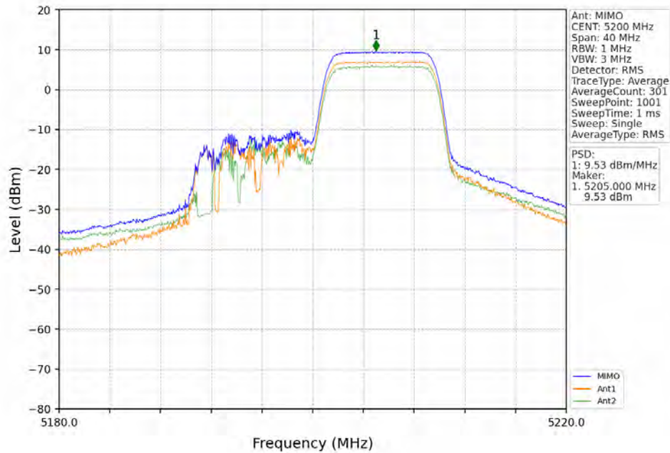
802.11ax(HEW20)_MCH_5200MHz_RU106_Right_MIMO_NTNV
