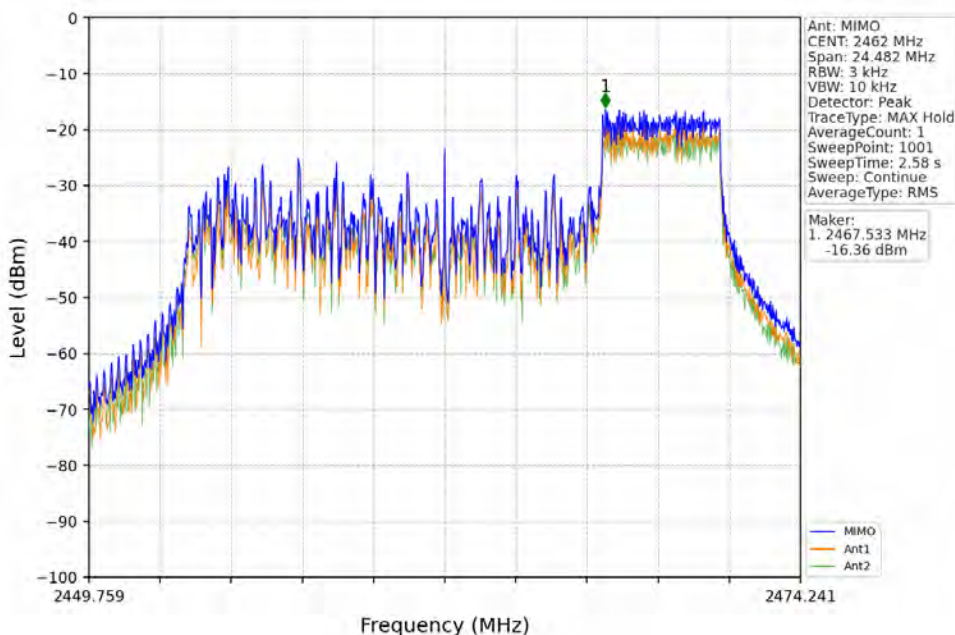
802.11ax(HEW20)_HCH_2462MHz_RU52_Right_MIMO_NTNV
