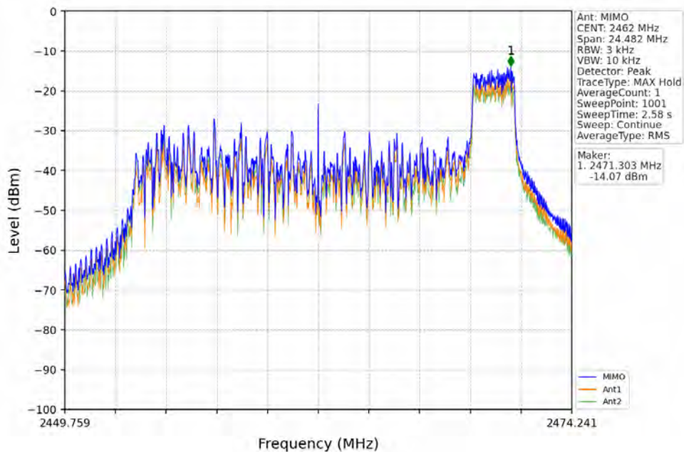
802.11ax(HEW20)_HCH_2462MHz_RU26_Right_MIMO_NTNV
