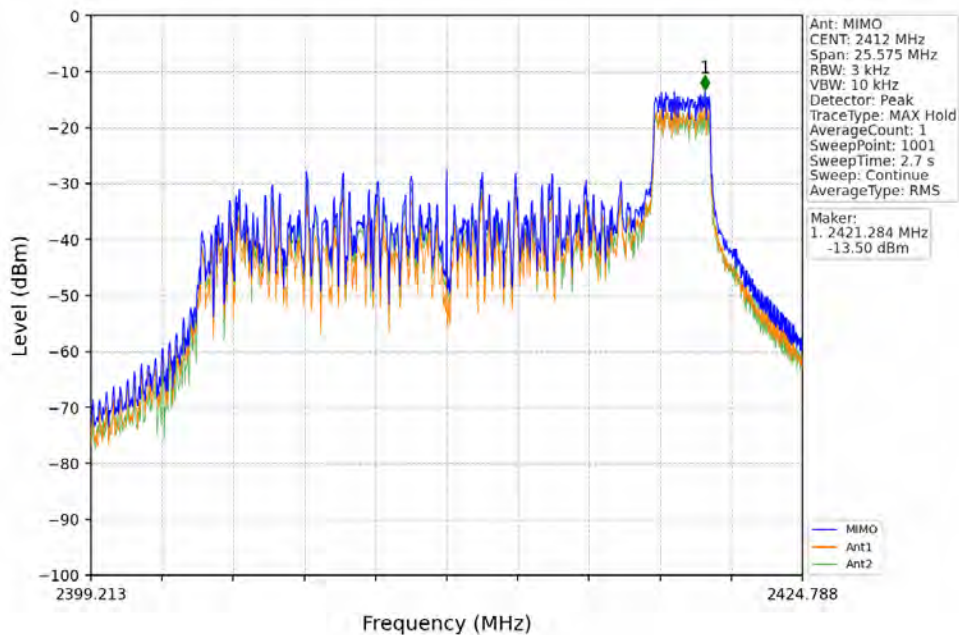
802.11ax(HEW20)_LCH_2412MHz_RU26_Right_MIMO_NTNV
