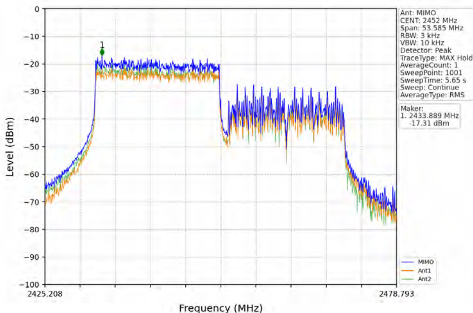
802.11ax(HEW40)_HCH_2452MHz_RU242_Left_MIMO_NTNV
