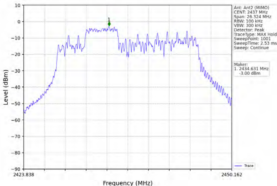
802.11ax(HEW20)_MCH_2437MHz_RU52_Mid_Ant2 (MIMO)_NTNV
