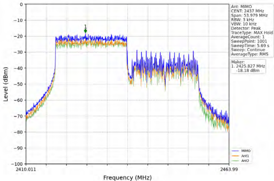
802.11ax(HEW40)_MCH_2437MHz_RU242_Right_MIMO_NTNV
