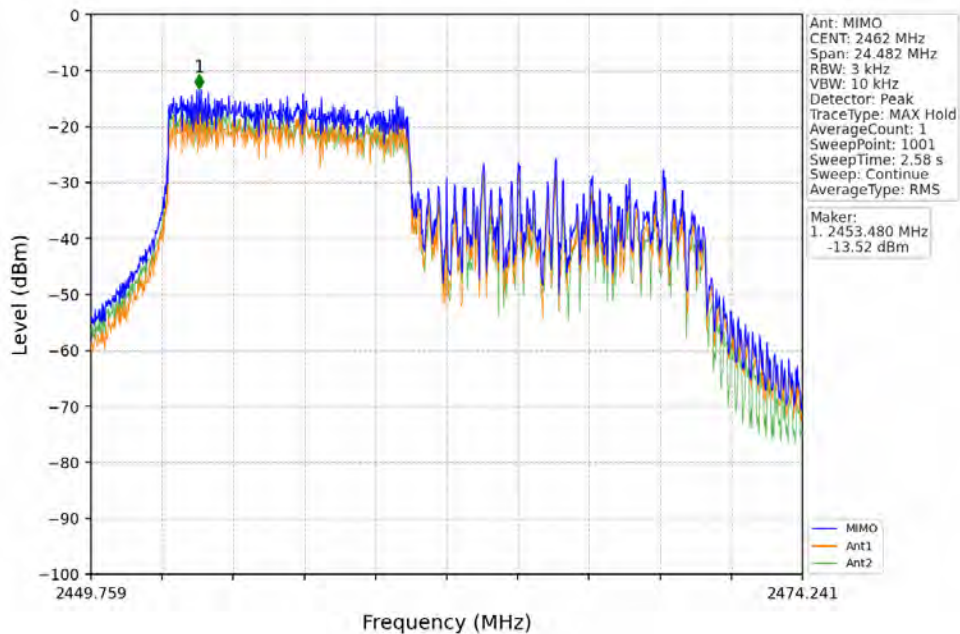
802.11ax(HEW20)_HCH_2462MHz_RU106_Right_MIMO_NTNV
