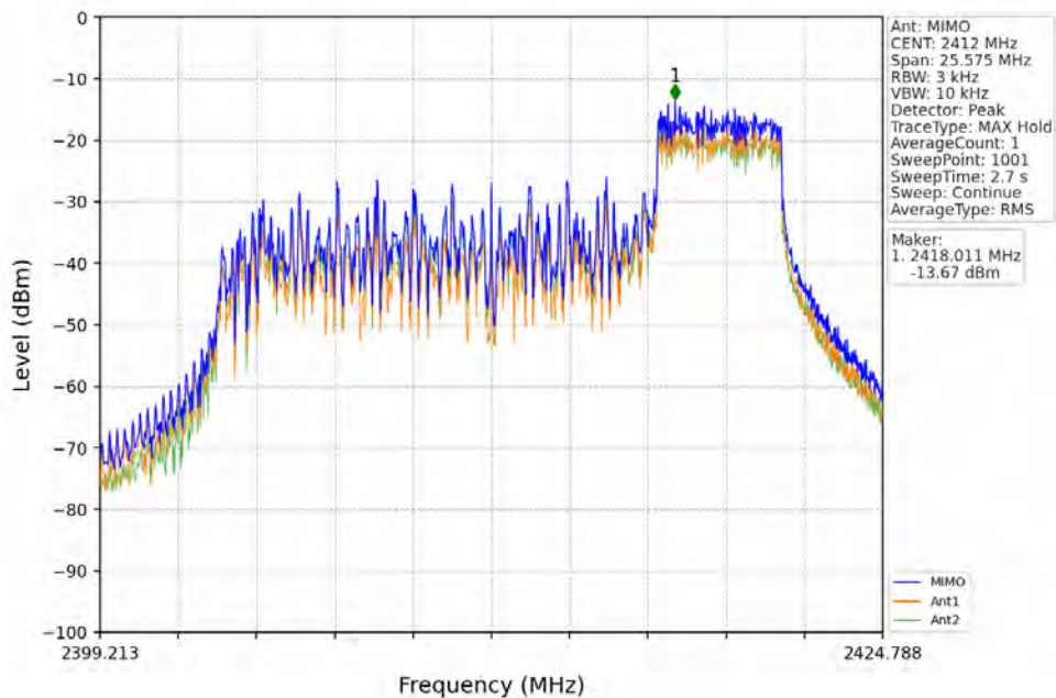
802.11ax(HEW20)_LCH_2412MHz_RU52_Right_MIMO_NTNV
