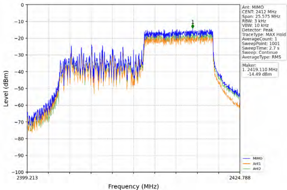
802.11ax(HEW20)_LCH_2412MHz_RU106_Right_MIMO_NTNV
