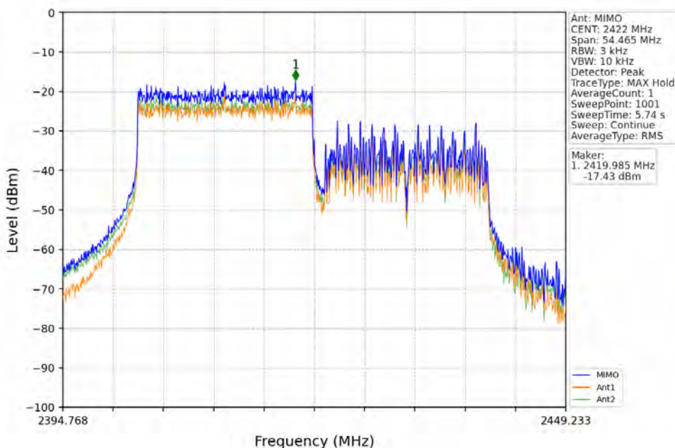
802.11ax(HEW40)_LCH_2422MHz_RU242_Left_MIMO_NTNV
