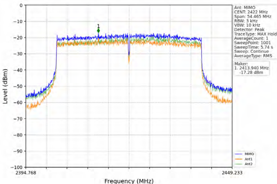
802.11ax(HEW40)_LCH_2422MHz_RU484_Left_MIMO_NTNV
