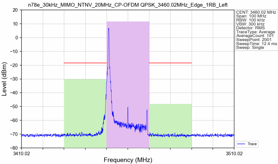
n78e_30kHz_MIMO_NTNV_20MHz_CP-OFDM QPSK_3460.02MHz_Edge_1RB_Left_Ant3
