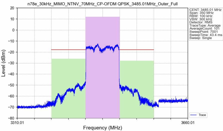
n78e_30kHz_MIMO_NTNV_70MHz_CP-OFDM QPSK_3485.01MHz_Outer_Full_Ant3
