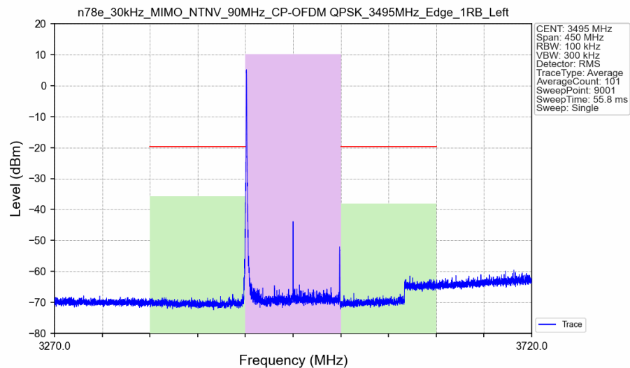
n78e_30kHz_MIMO_NTNV_90MHz_CP-OFDM QPSK_3495MHz_Edge_1RB_Left_Ant3
