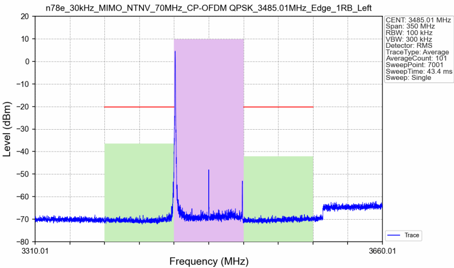
n78e_30kHz_MIMO_NTNV_70MHz_CP-OFDM QPSK_3485.01MHz_Edge_1RB_Left_Ant3
