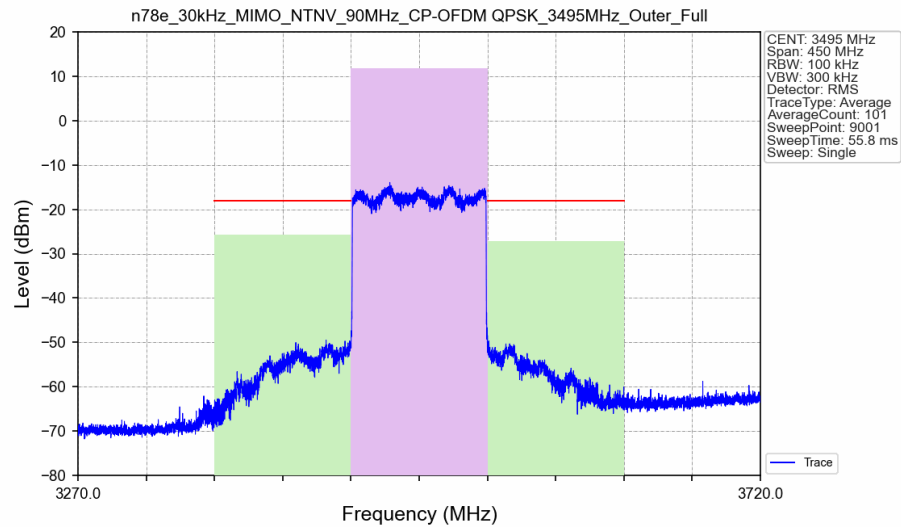
n78e_30kHz_MIMO_NTNV_90MHz_CP-OFDM QPSK_3495MHz_Outer_Full_Ant3
