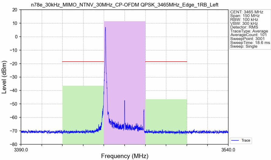
n78e_30kHz_MIMO_NTNV_30MHz_CP-OFDM QPSK_3465MHz_Edge_1RB_Left_Ant3
