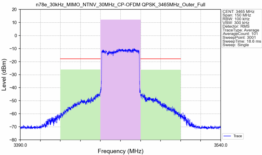
n78e_30kHz_MIMO_NTNV_30MHz_CP-OFDM QPSK_3465MHz_Outer_Full_Ant3
