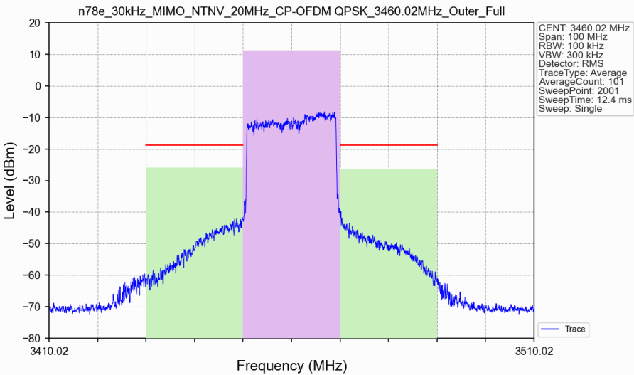
n78e_30kHz_MIMO_NTNV_20MHz_CP-OFDM QPSK_3460.02MHz_Outer_Full_Ant3
