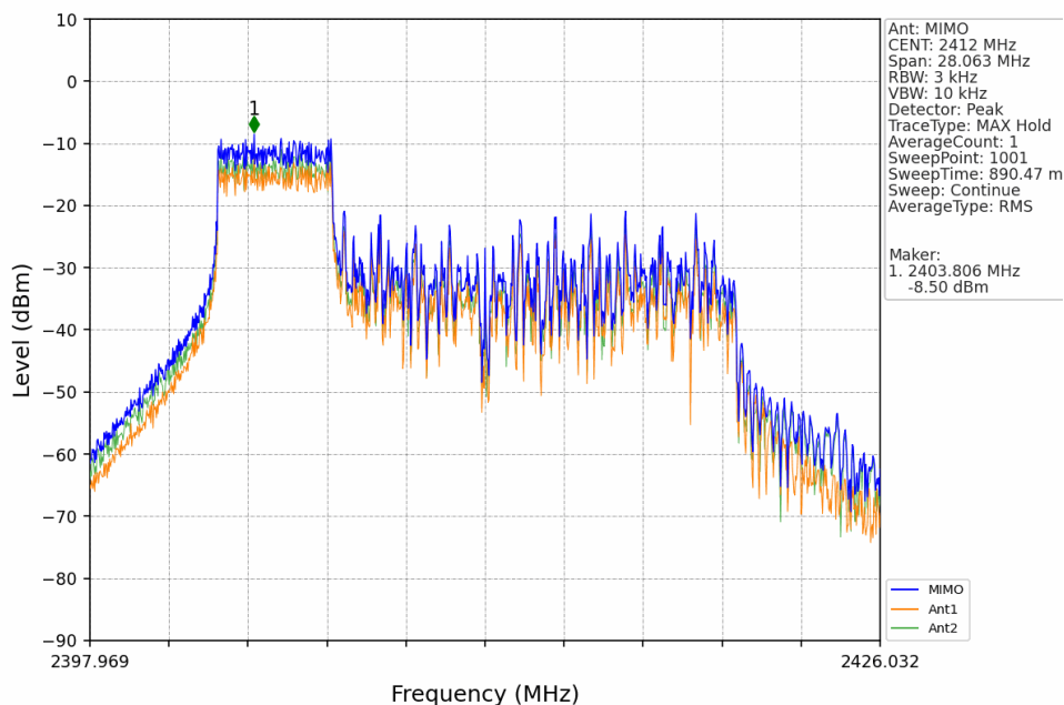
802.11ax(HEW20)_LCH_2412MHz_RU52_Left_MIMO_NTNV
