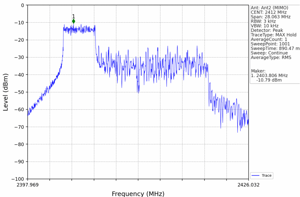
802.11ax(HEW20)_LCH_2412MHz_RU52_Left_MIMO_NTNV
