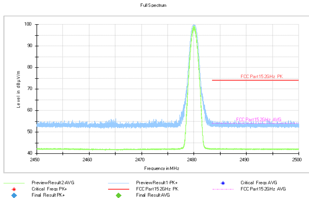
Fig.14. Frequency Band Edges: GFSK, Channel 78, Hopping Off, ch11, 2.45 GHz - 2.50GHz
