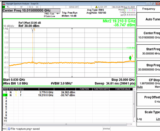
n78(3700-3800MHz) (30MHz-20GHz) 60M DFT-s-OFDM BPSK Inner_1RB_Right Mid
