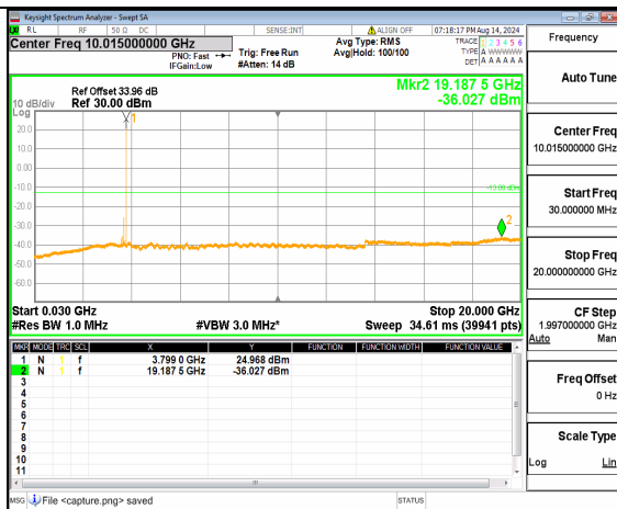
n78(3700-3800MHz) (30MHz-20GHz) 100M DFT-s-OFDM QPSK Inner_1RB_Right Mid
