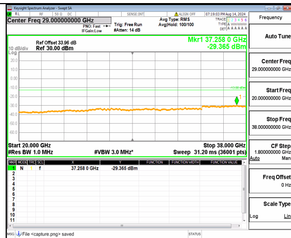
n78(3700-3800MHz) (20GHz-38GHz) 100M DFT-s-OFDM QPSK Inner_1RB_Right Mid
