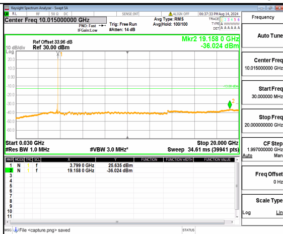
n78(3700-3800MHz) (30MHz-20GHz) 70M DFT-s-OFDM BPSK Inner_1RB_Right High
