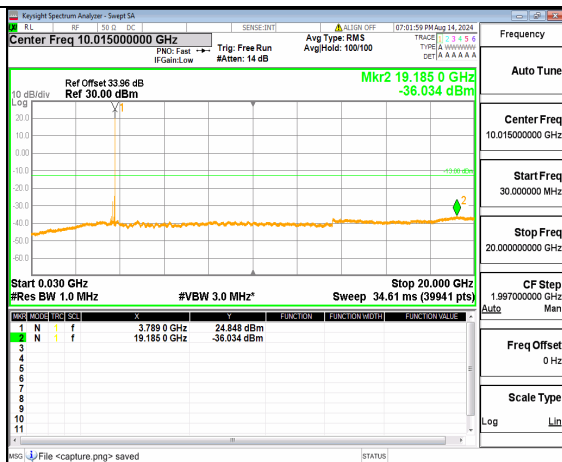
n78(3700-3800MHz) (30MHz-20GHz) 90M DFT-s-OFDM QPSK Inner_1RB_Right Low
