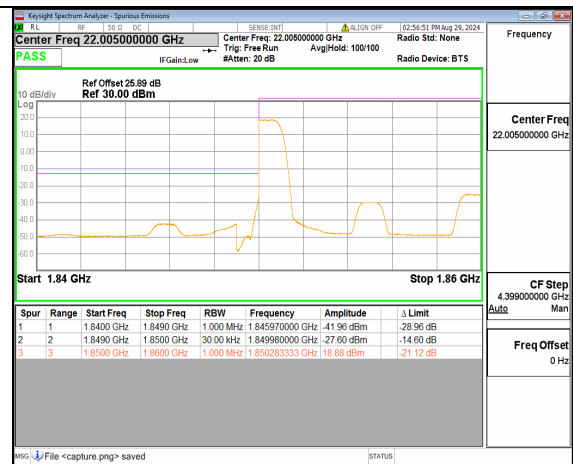
n2 10M DFT-s-OFDM 16QAM Edge_1RB_Left Low
