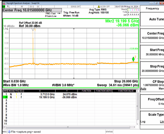
n78(3700-3800MHz) (30MHz-20GHz) 80M DFT-s-OFDM BPSK Inner_1RB_Left Mid
