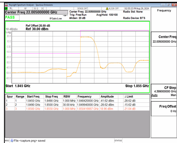
n2 5M DFT-s-OFDM 16QAM Edge_1RB_Left Low
