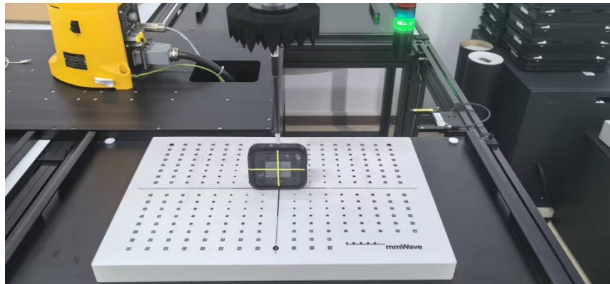
Top Side (Test distance: 2mm)
