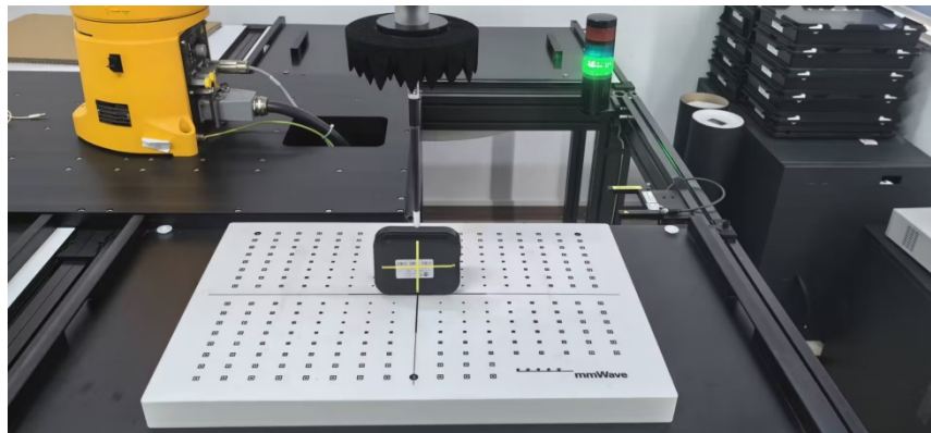
Bottom Side (Test distance: 2mm)
