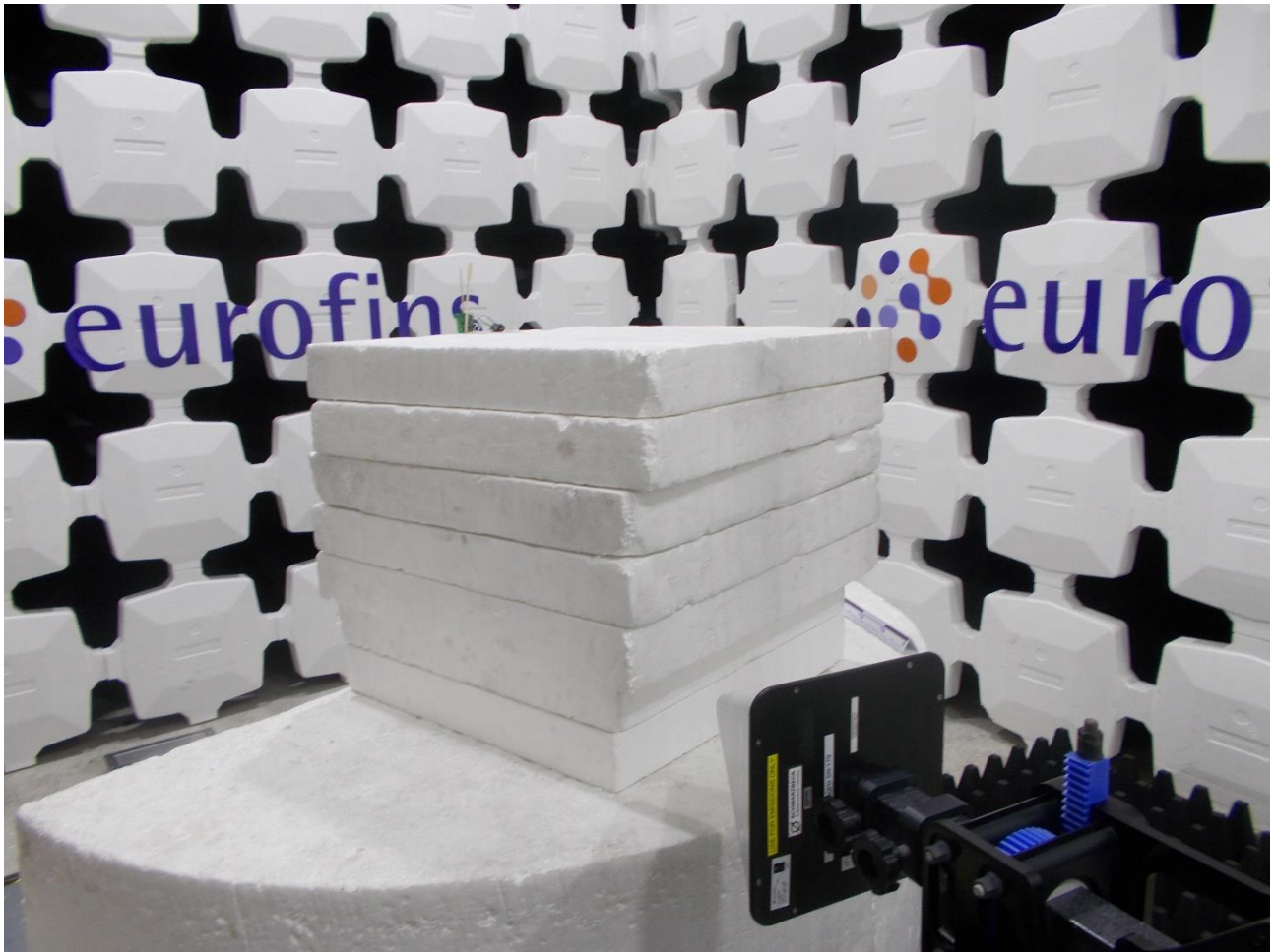
Radiated electric field emissions > 1GHz
