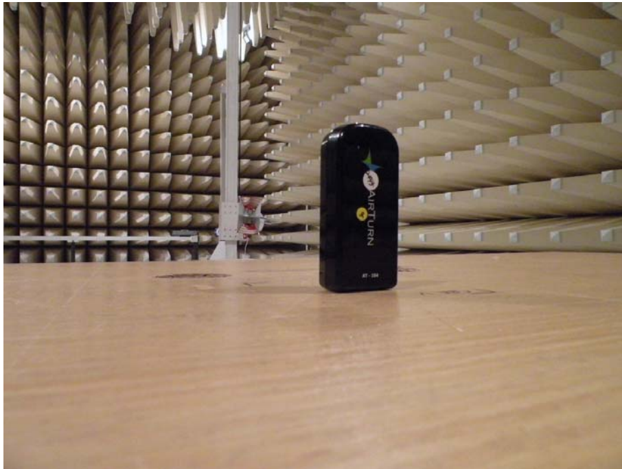
< X-axis Radiated emission Test >
