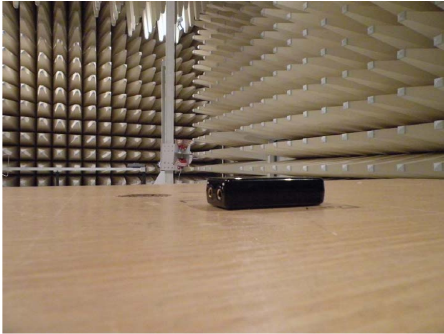
< Z-axis Radiated emission Test >
