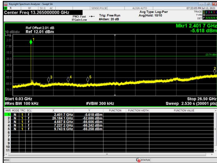
30MHz~26.5GHz
