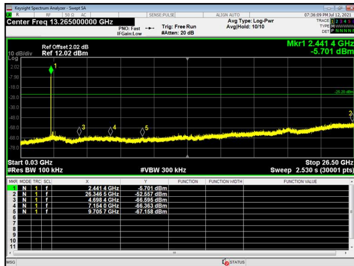
30MHz~26.5GHz
