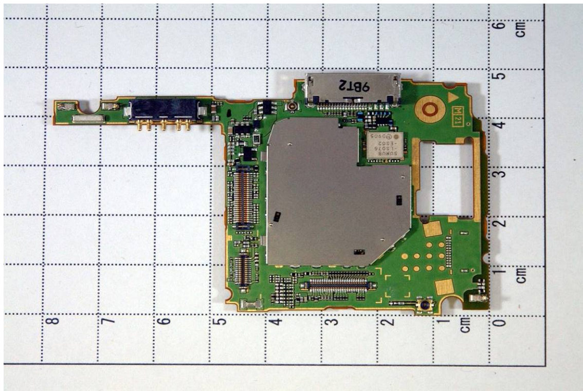
Lower PCB with shielding (Back)
