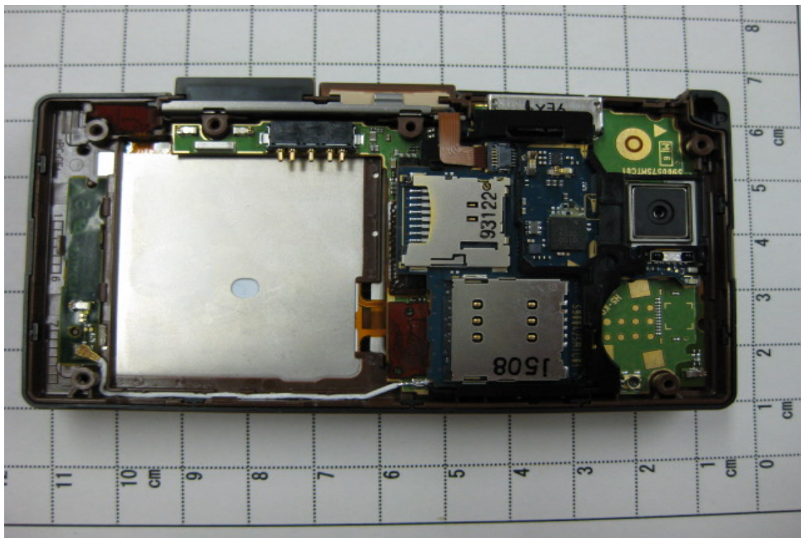
Lower Case (inside) with Lower PCB and Sub PCB
