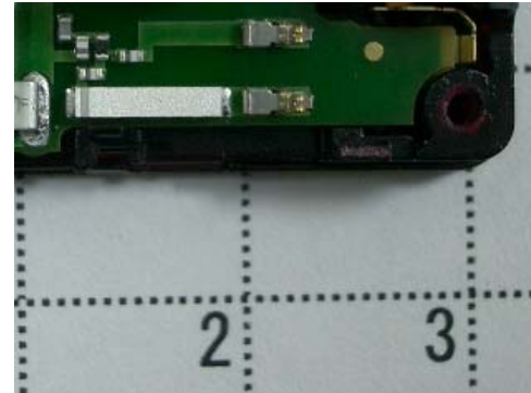
Sub antenna (Chip)
