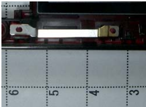
Bluetooth antenna
