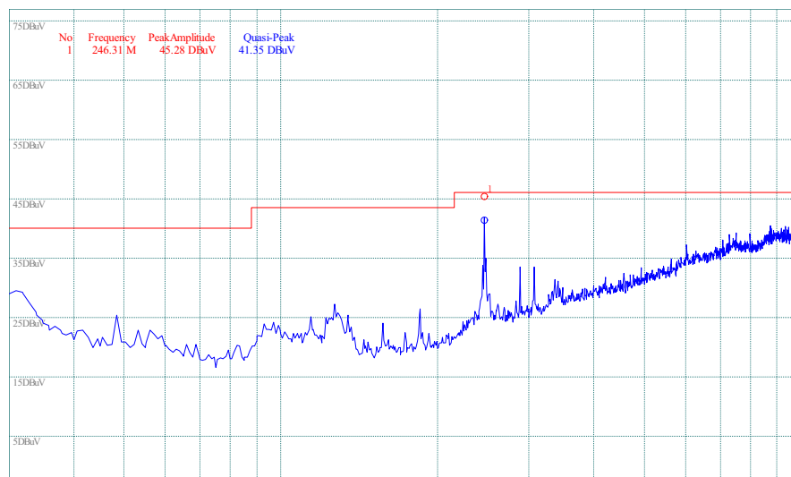
(Plot B: Test Antenna Horizontal)
