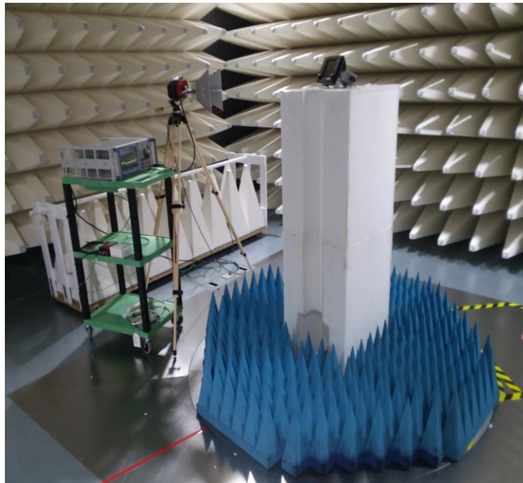
Figure B5. Radiated Setup
