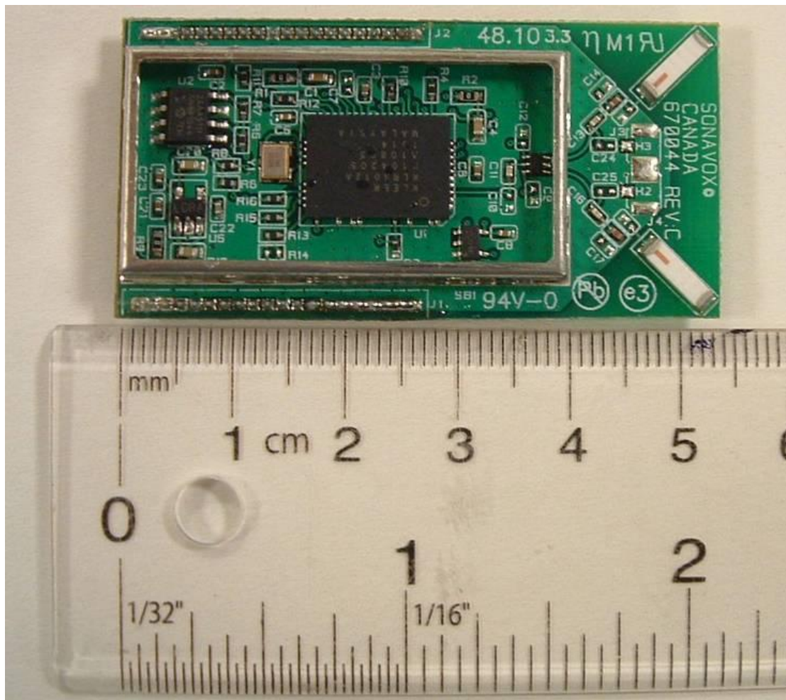
EUT – Top view (shield removed)
