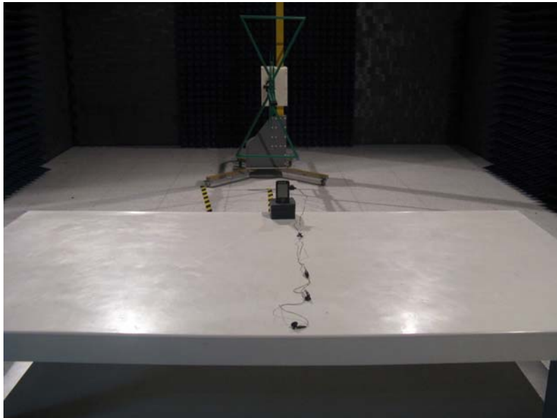
Radiated Emission Test Setup Photo
