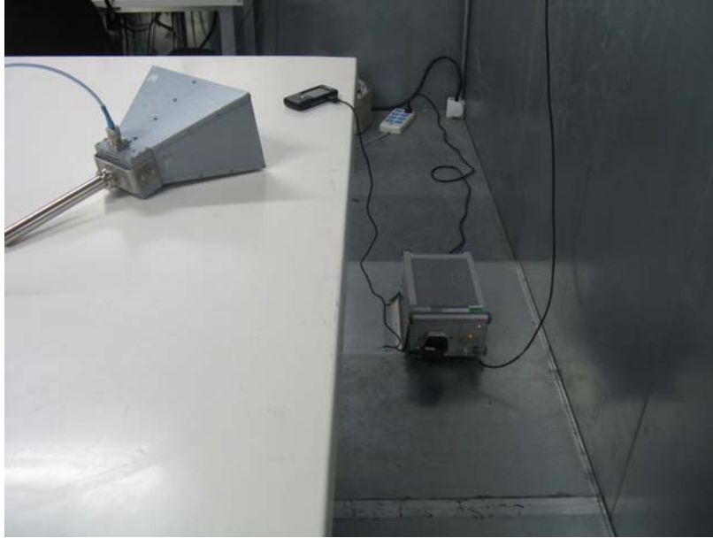
Conducted Emission Test Setup Photo
