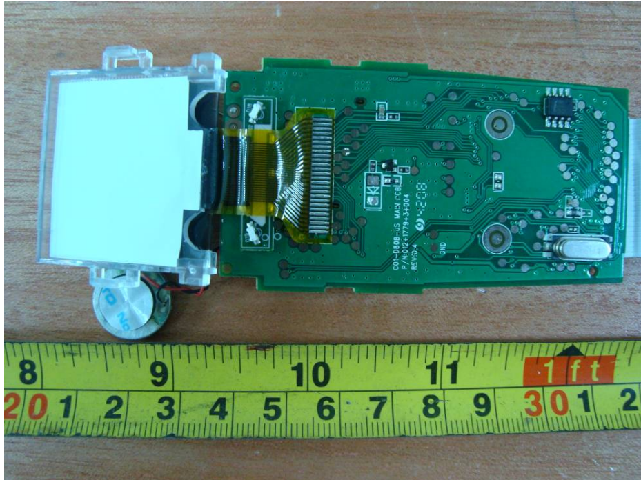
EUT – Main Board Bottom Components View (With Shielded Cover)
