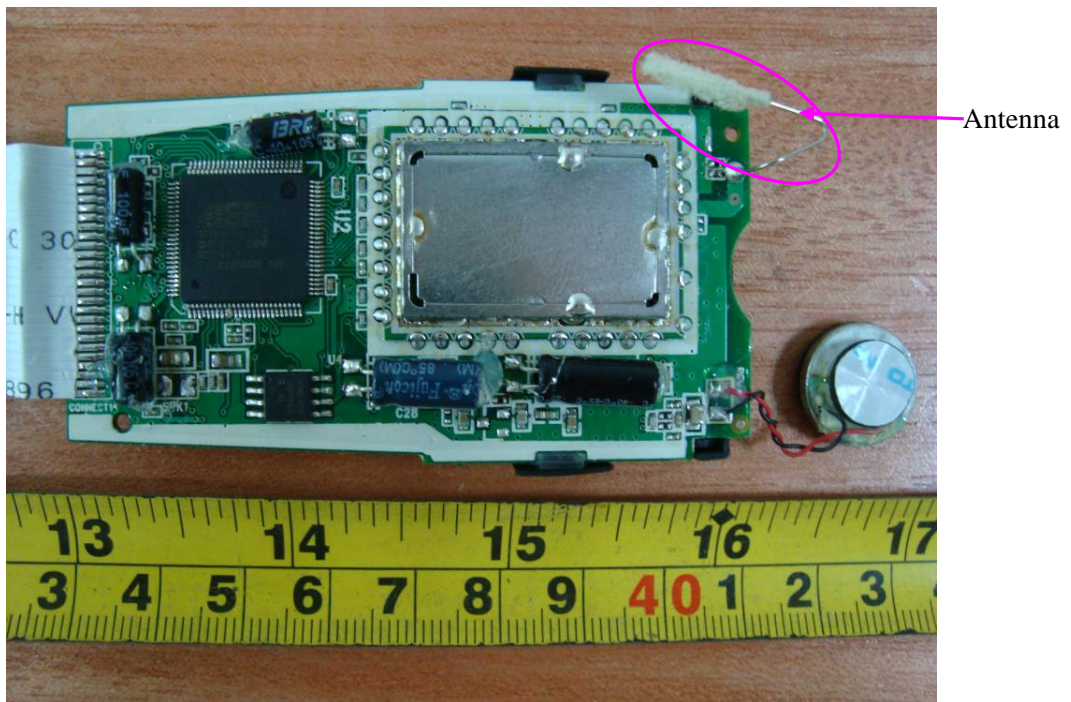
EUT – Main Board Bottom Components View (With Shielded Cover)
