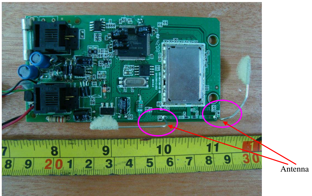
EUT – Main Board Top View (With Shielded Cover)
