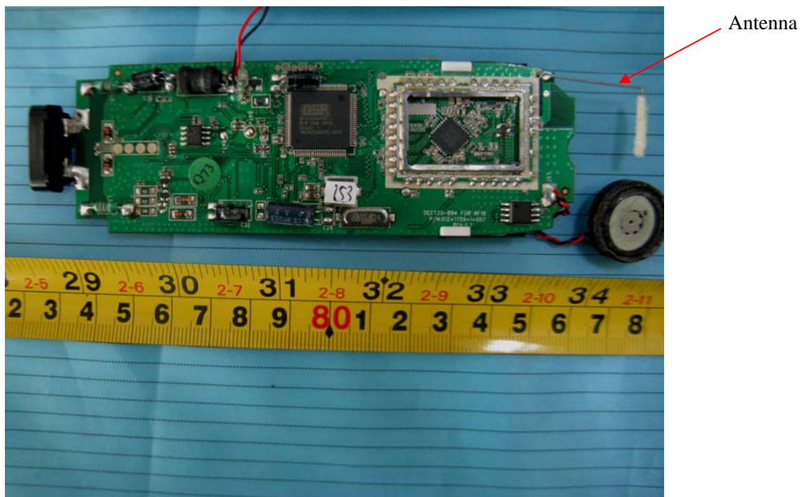
EUT – Main Board Bottom Components View (Without Shielded Cover)
