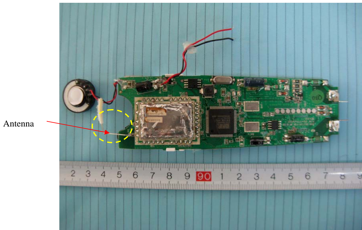
EUT – Main Board Bottom Components View (With Shielding)
