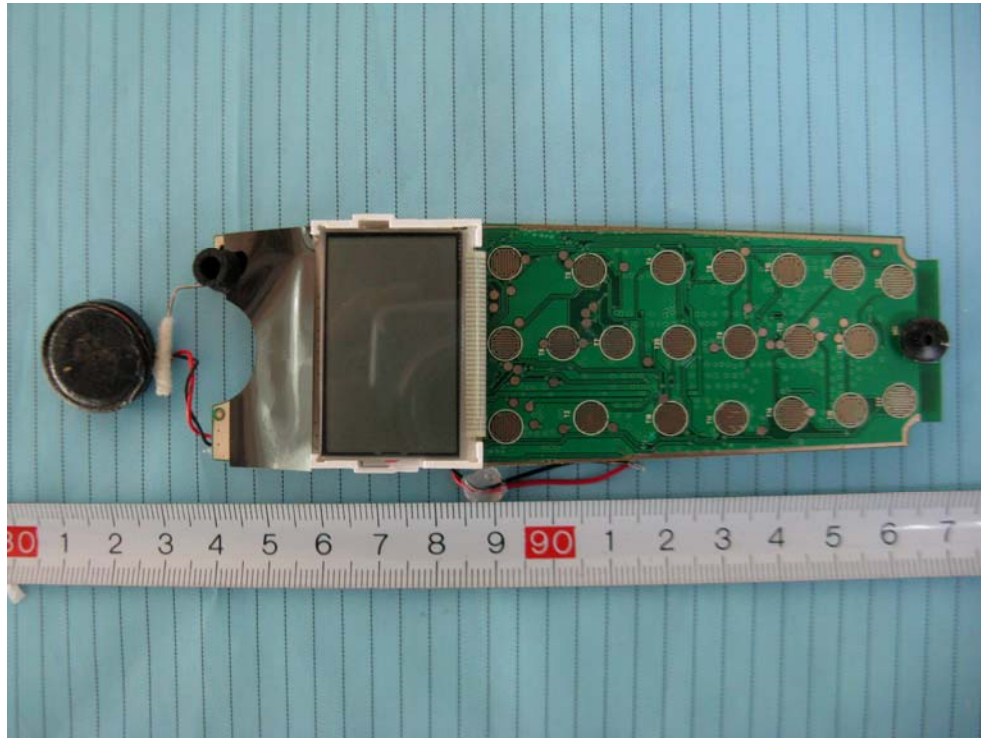
EUT – Main Board Bottom Components View (With Shielding)
