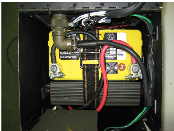
BATTERY SYSTEM
