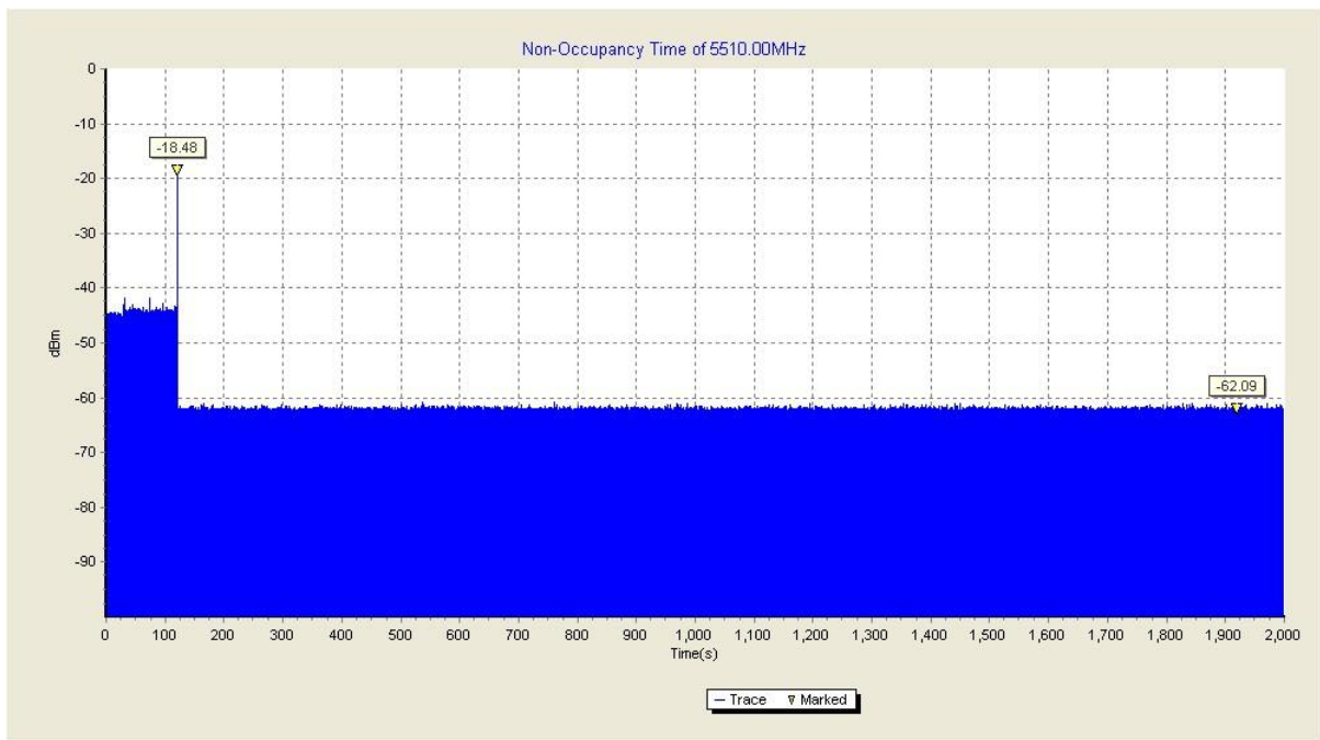
Fig.6 Non-Occupancy Period (HT40 Frequency Band: 5470MHz ~ 5725MHz)
