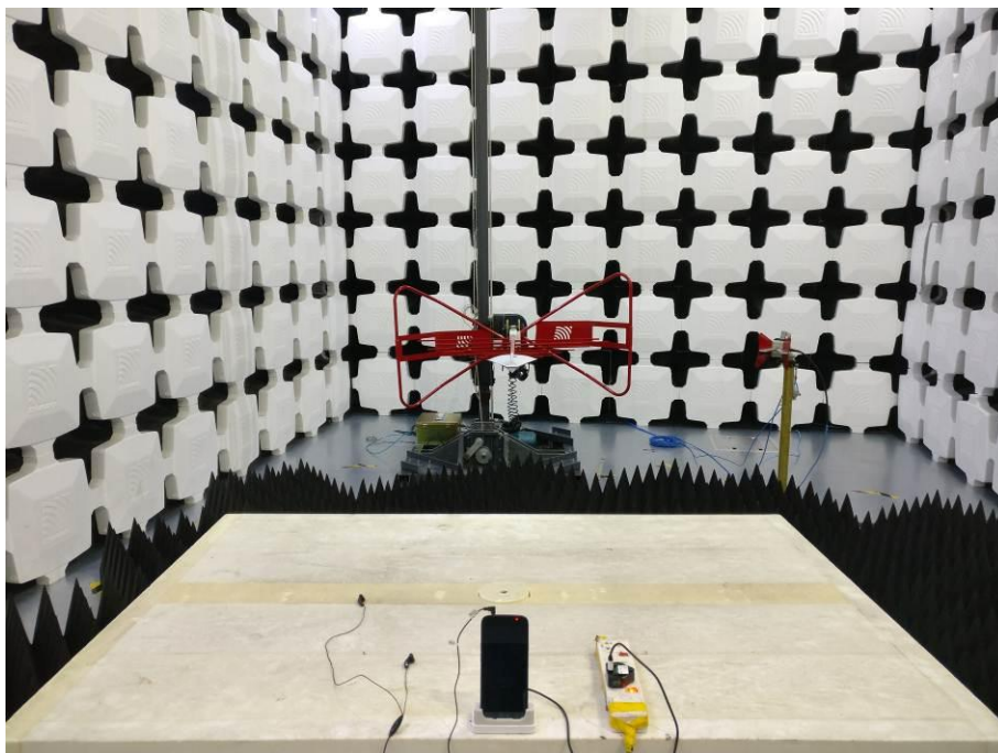
6. Radiated Emissions (Part 15B Charging mode 2) (1GHz-18GHz)
