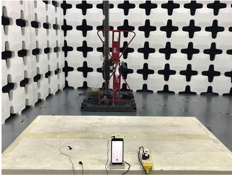
5. Radiated Emissions (Part 15B Charging mode 2) (30MHz-1GHz)
