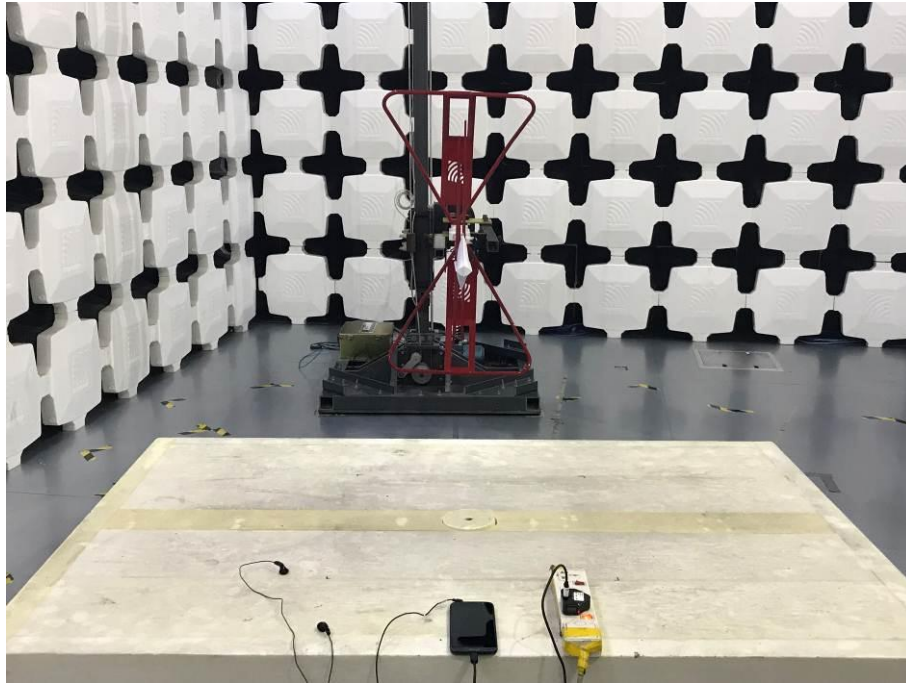
3. Radiated Emissions (Part 15B Charging mode 1) (30MHz-1GHz)
