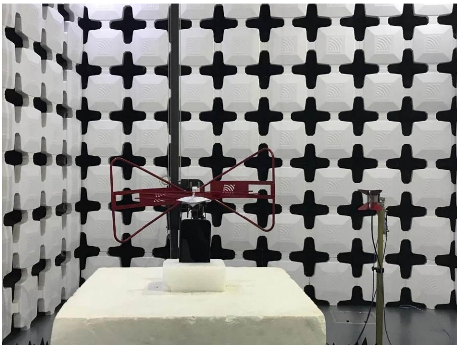
12. Radiated Emissions (Part 22/24/27) (30MHz-18GHz)
