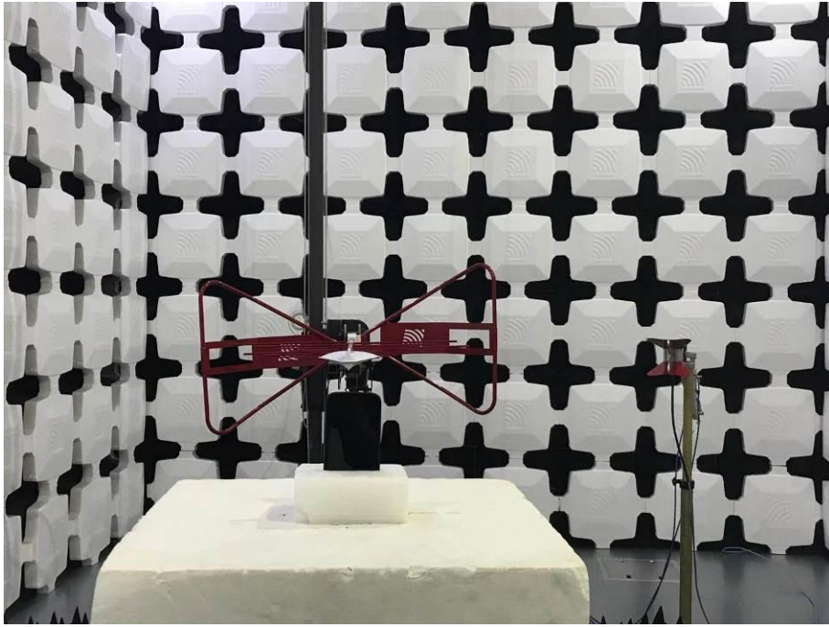
9. Radiated Emissions (Part 15C&E) (1-18GHz)
