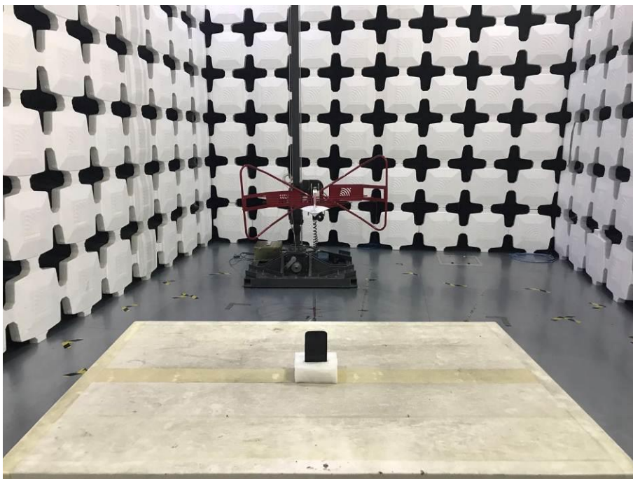
8. Radiated Emissions (Part 15C&E) (30MHz-1GHz)
