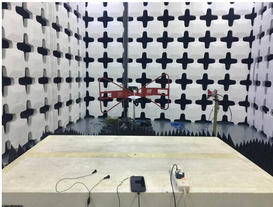
4. Radiated Emissions (Part 15B Charging mode 1) (1GHz-18GHz)
