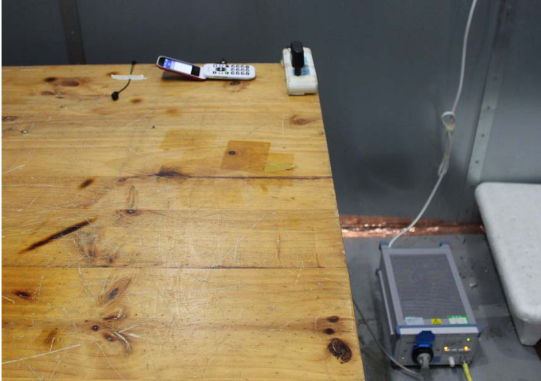
Picture 2 Conducted Emission Test Setup
