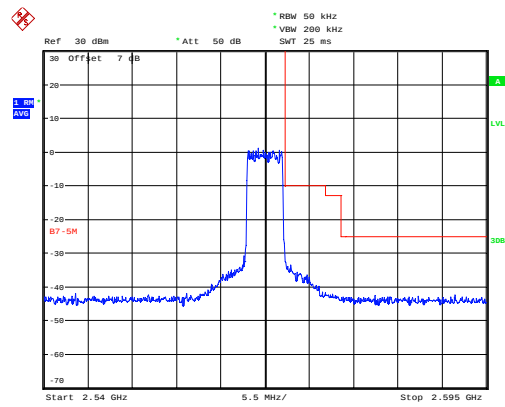
LTE Band 7 QPSK 5MHz CH-High, 100%RB
