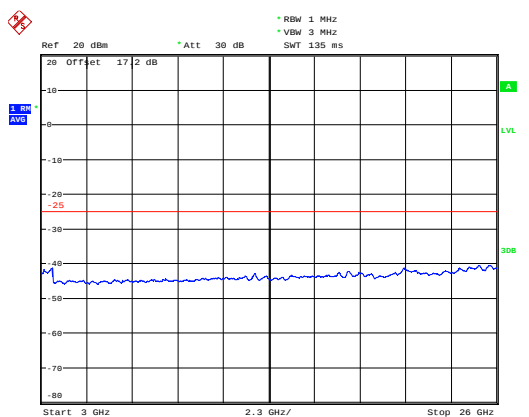
LTE Band 7 5MHz CH-Low 3GHz~26GHz
