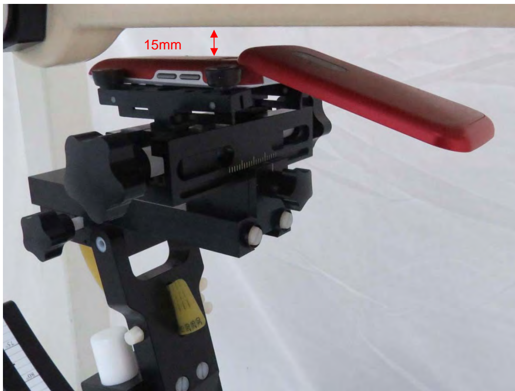
Picture 10: Back Side Open, the distance from handset to the bottom of the Phantom is 15mm
