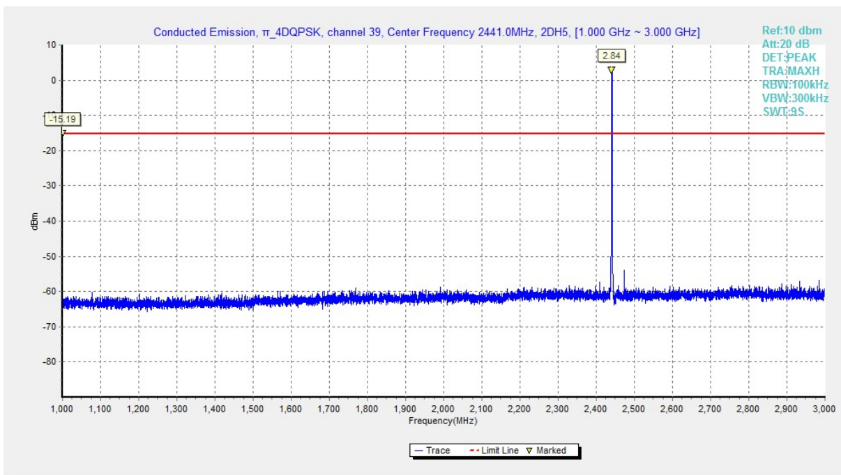
Fig. 21 Conducted Spurious Emission ( \pi/4 DQPSK, Ch39, 1GHz-3 GHz)
