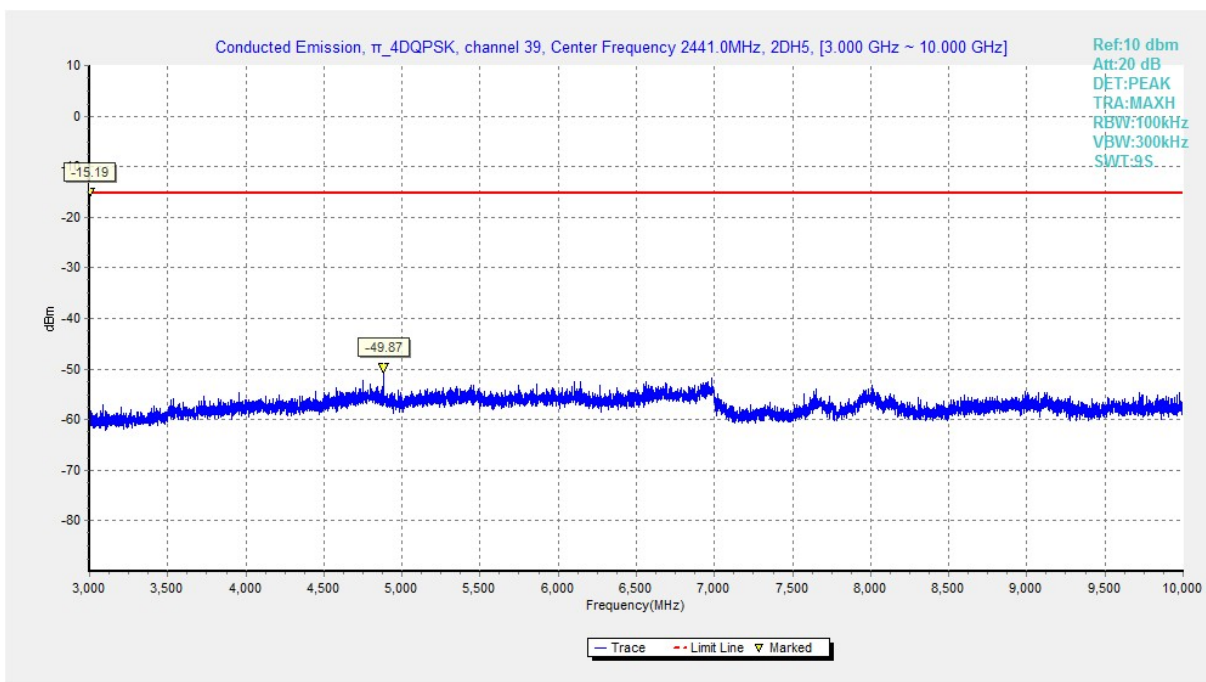
Fig. 22 Conducted Spurious Emission ( \pi/4 DQPSK, Ch39, 3GHz-10 GHz)
