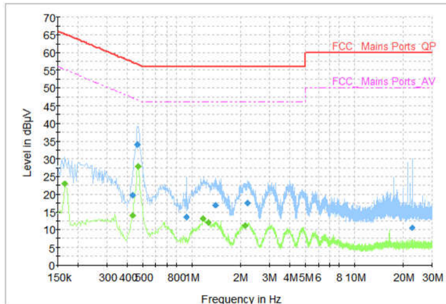
Fig.31 AC Powerline Conducted Emission (Traffic)
