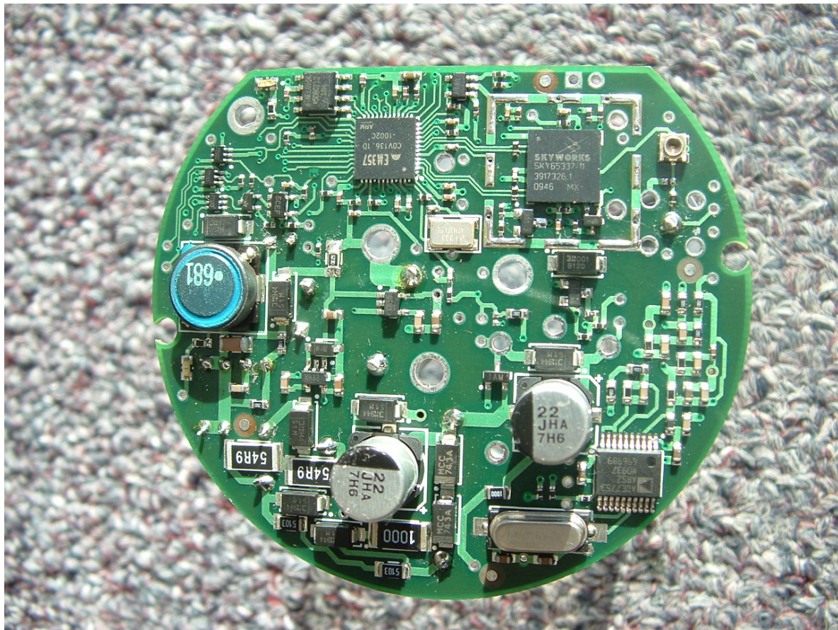
Photograph of PC Board foil side: RF cover removed
