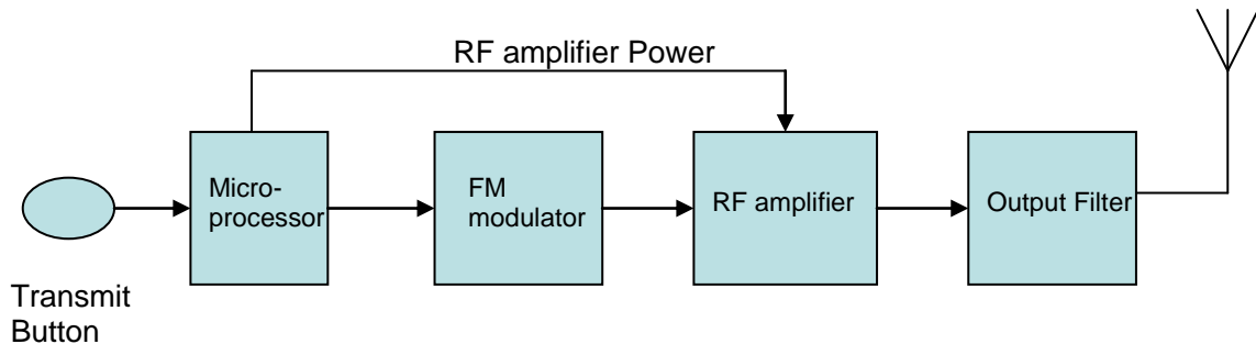
Transmitter block diagram
