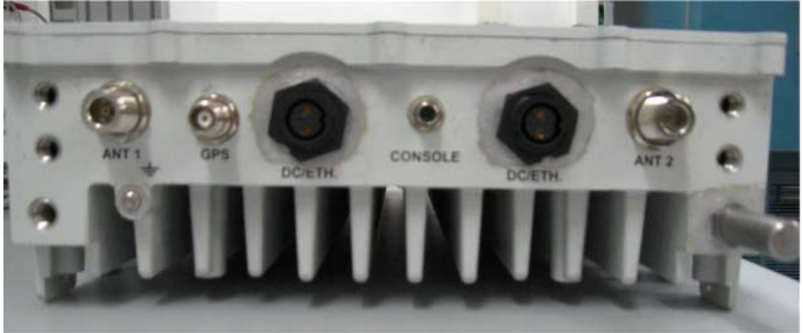
Photograph No.1 Base station WiN7037-2 front view
