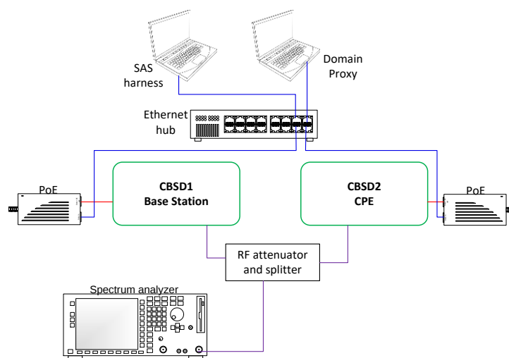
Figure 3.6-1: Setup diagram
