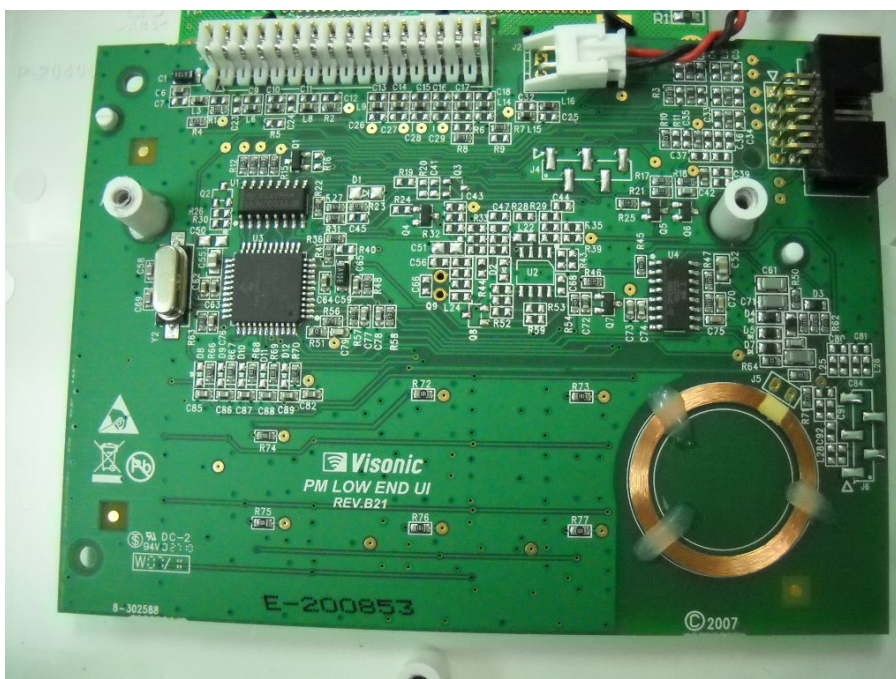
Photograph 7.2.1 Antenna assembly
