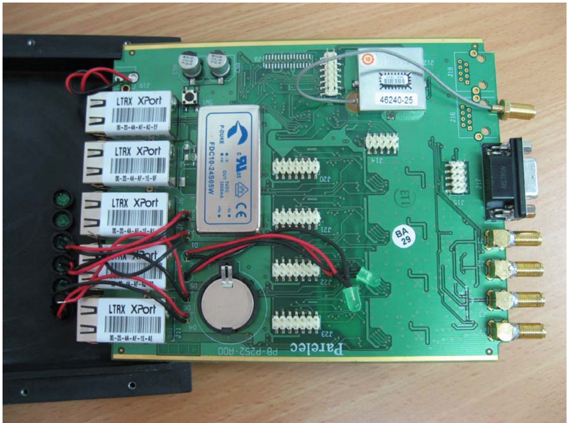
Base station
