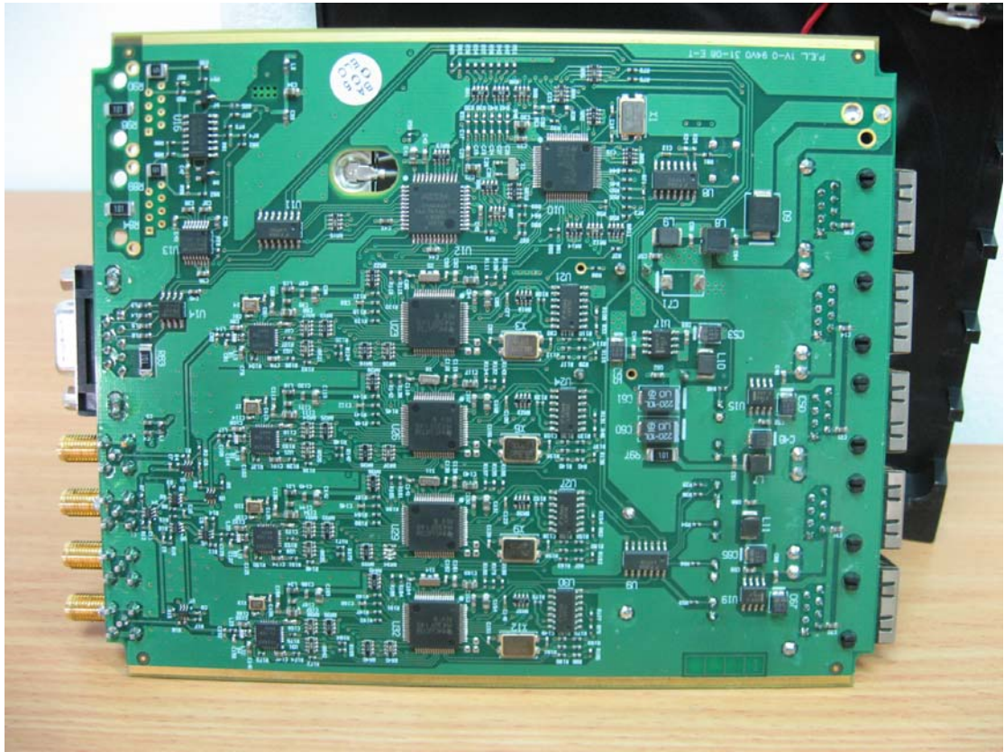
Base Station
