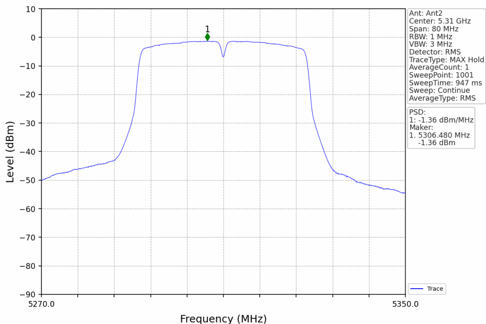
802.11n(HT40)_HCH_5310MHz_Ant2_NTNV
