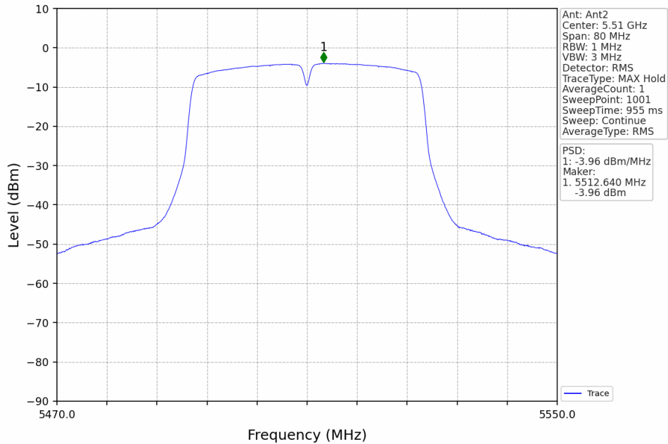
802.11ac(VHT40)_LCH_5510MHz_MIMO_NTNV
