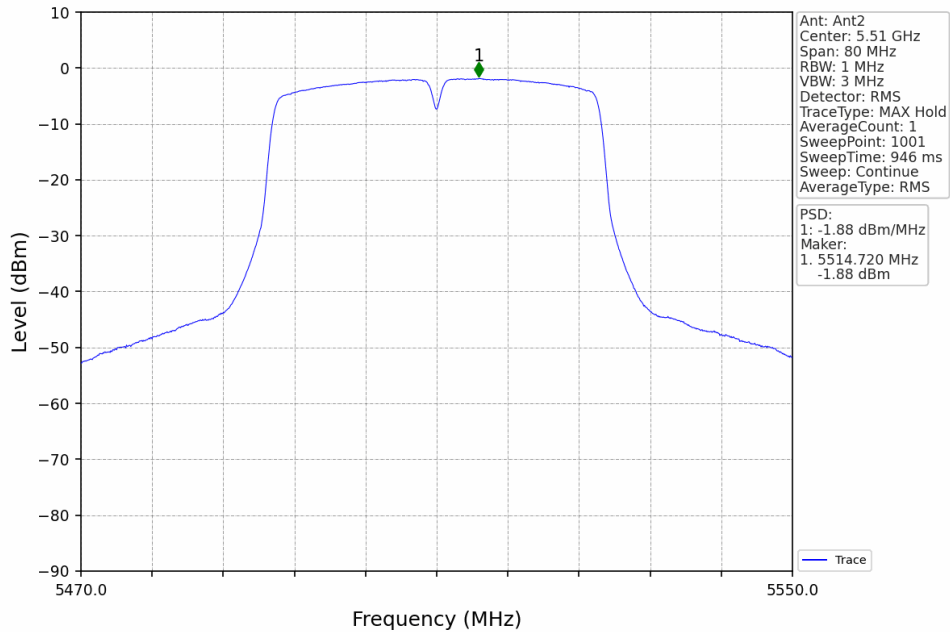
802.11n(HT40)_LCH_5510MHz_MIMO_NTNV
