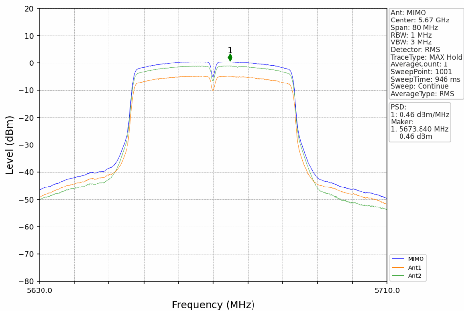
802.11n(HT40)_HCH_5670MHz_MIMO_NTNV
