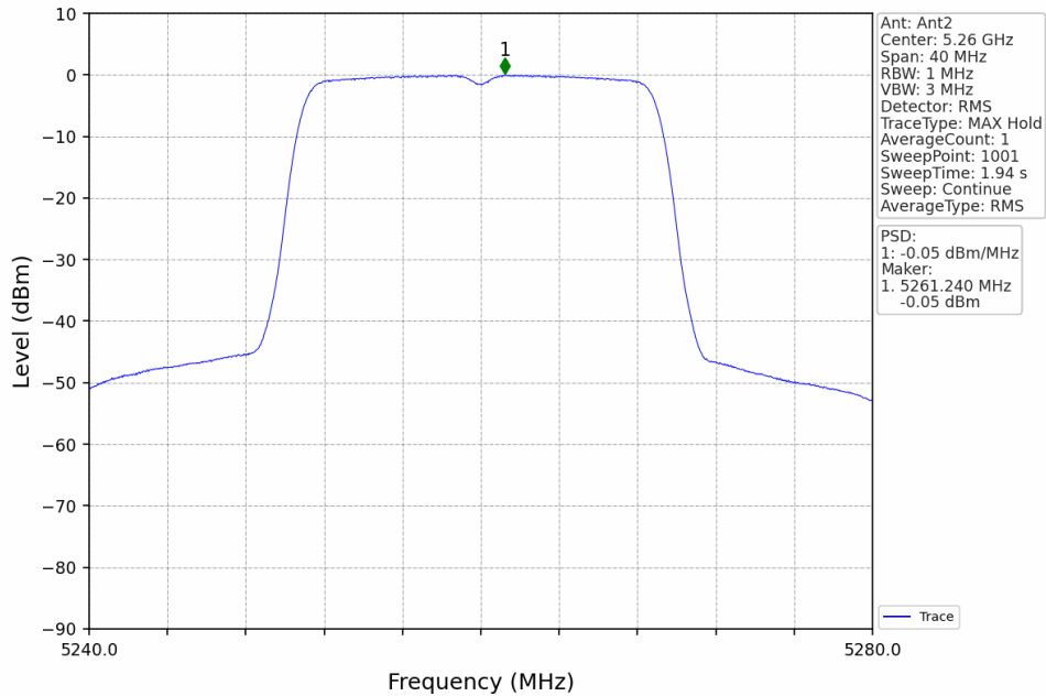
802.11ac(VHT20)_LCH_5260MHz_MIMO_NTNV
