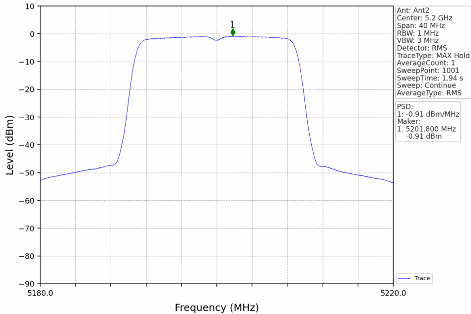
802.11ac(VHT20)_MCH_5200MHz_MIMO_NTNV
