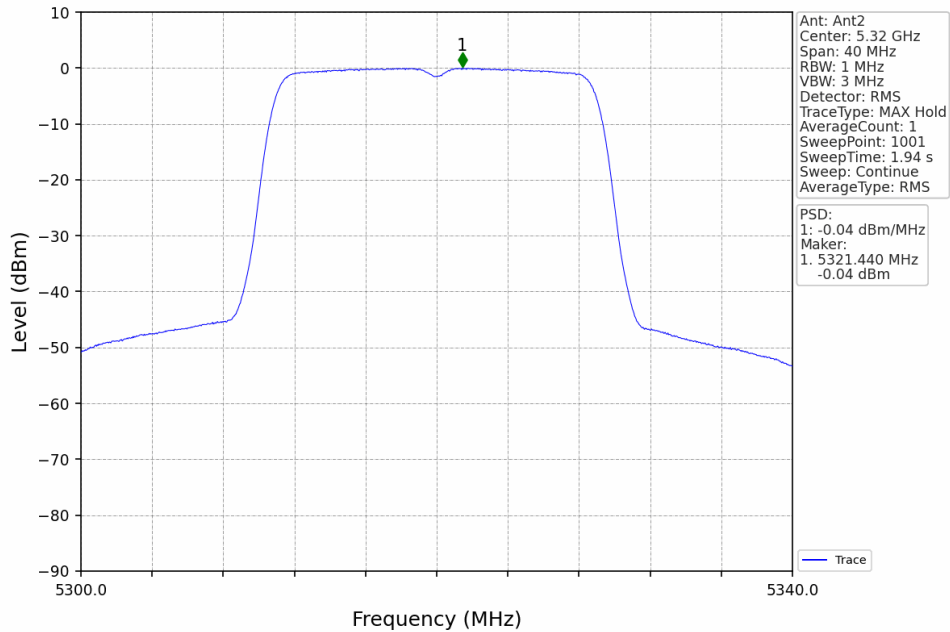
802.11ac(VHT20)_HCH_5320MHz_MIMO_NTNV
