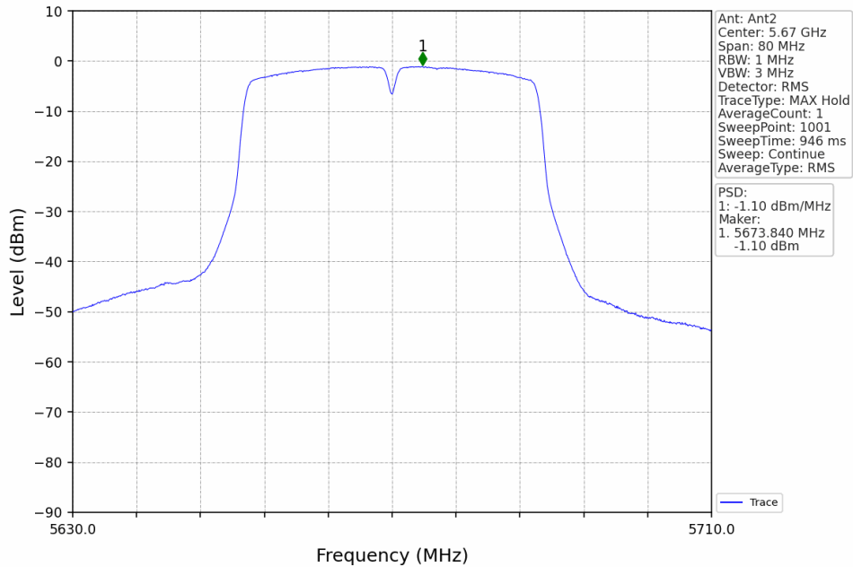
802.11n(HT40)_HCH_5670MHz_MIMO_NTNV
