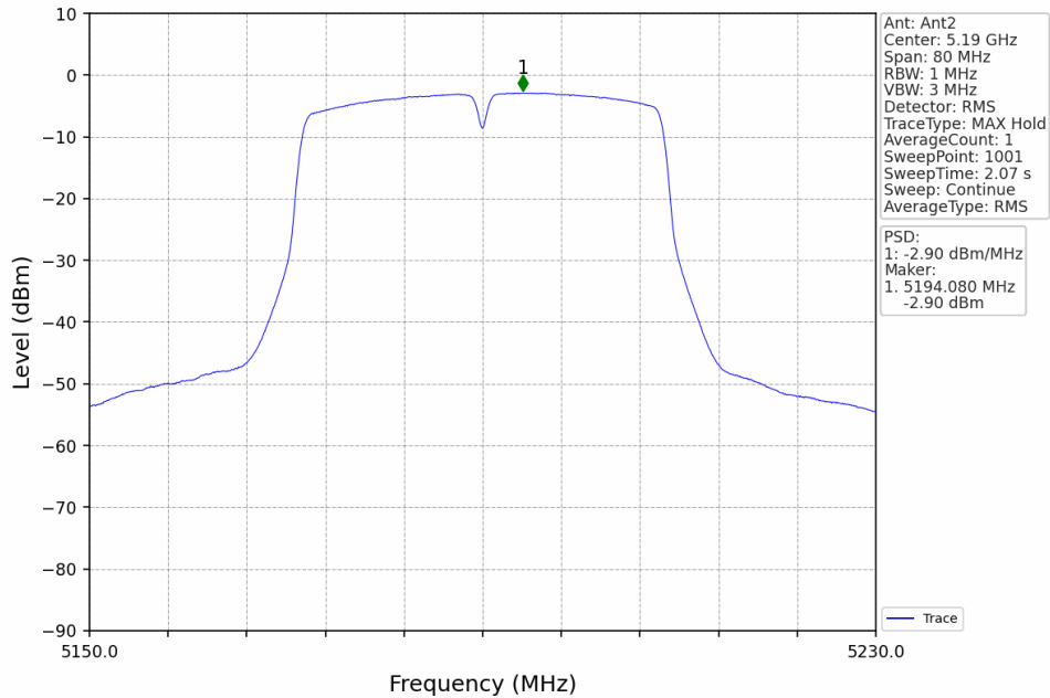
802.11n(HT40)_LCH_5190MHz_MIMO_NTNV
