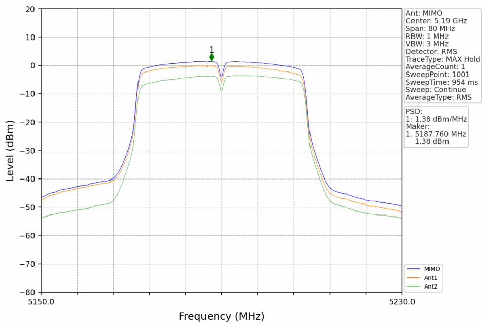
802.11ac(VHT40)_LCH_5190MHz_MIMO_NTNV
