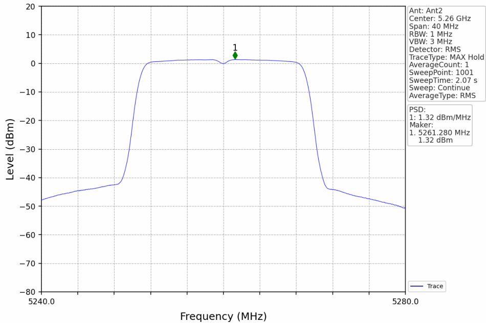
802.11n(HT20)_LCH_5260MHz_MIMO_NTNV
