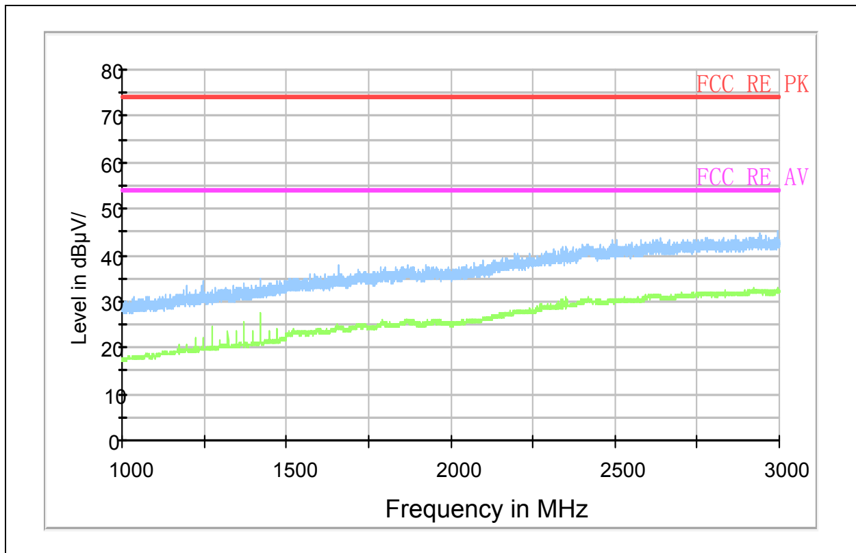
Radiated Emission from 1GHz to 3GHz
