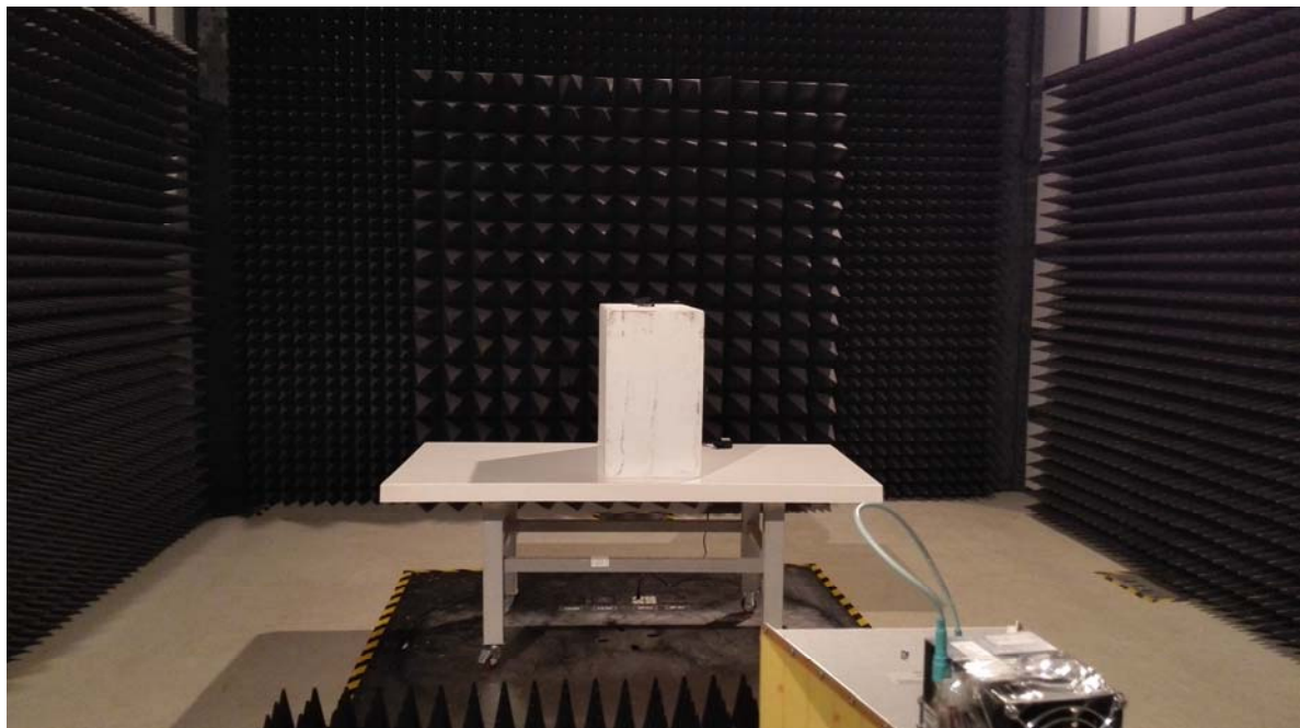
Spurious Emissions View (Above 1 GHz)
