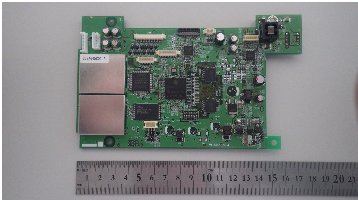
Main control board (Back side)
