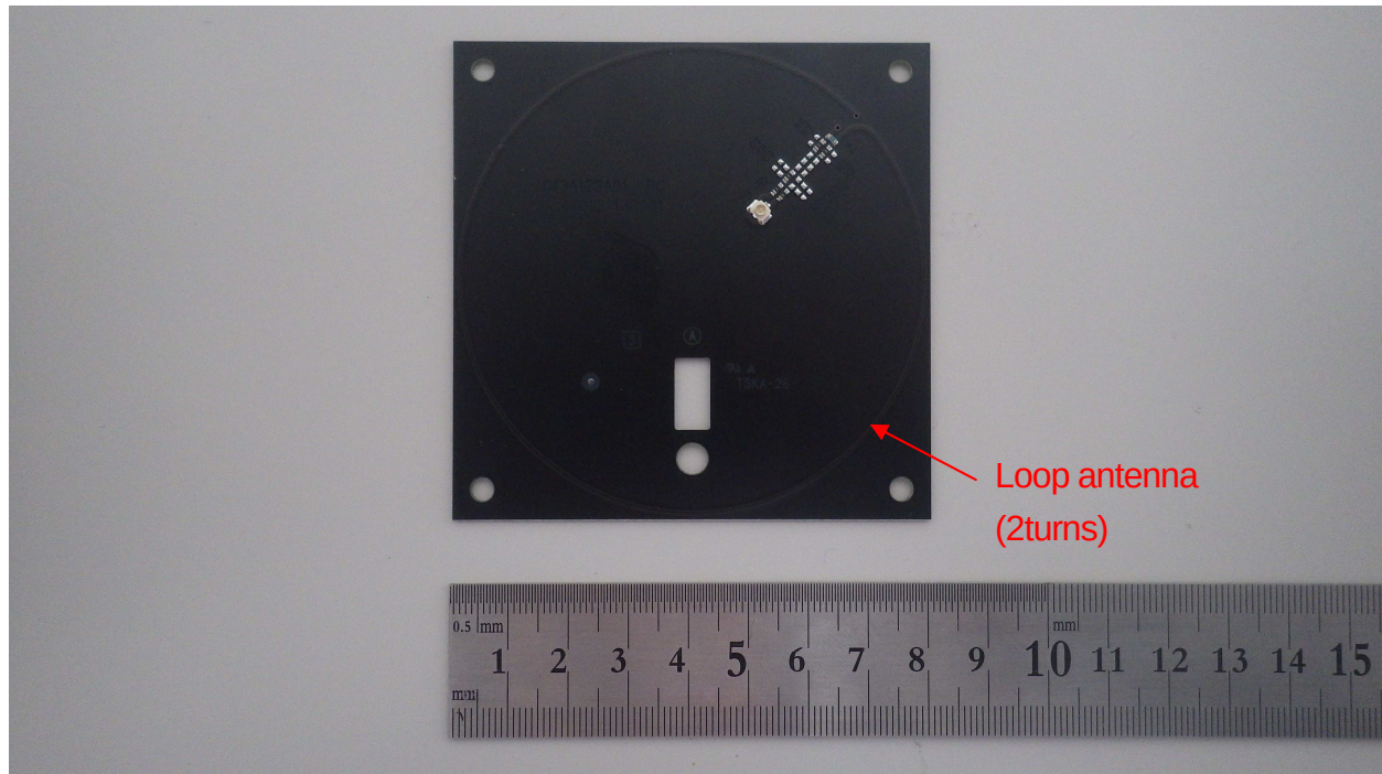
Loop antenna board (Lower antenna) (Front side)
