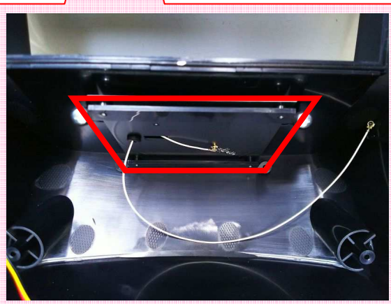
Loop antenna board (Lower antenna)
