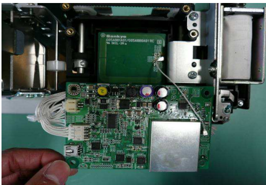
Wireless part circuit and antenna circuit
