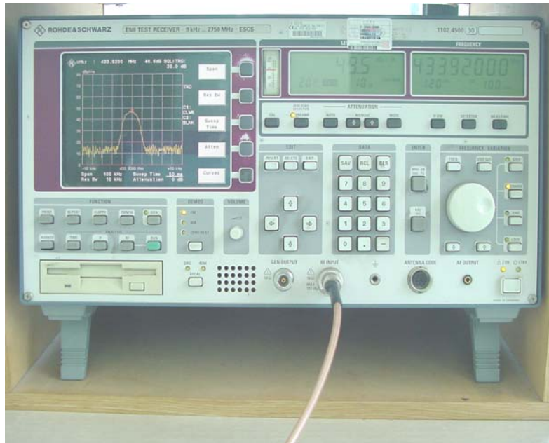
[ Fundamental signal detected in Test receiver_ Reading value ]
