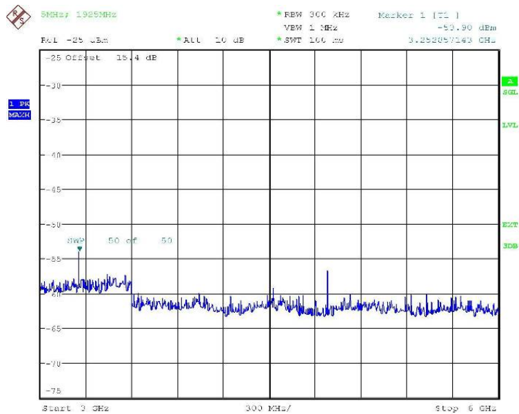
Figure 6-10: Conducted Emissions (middle frequency)
