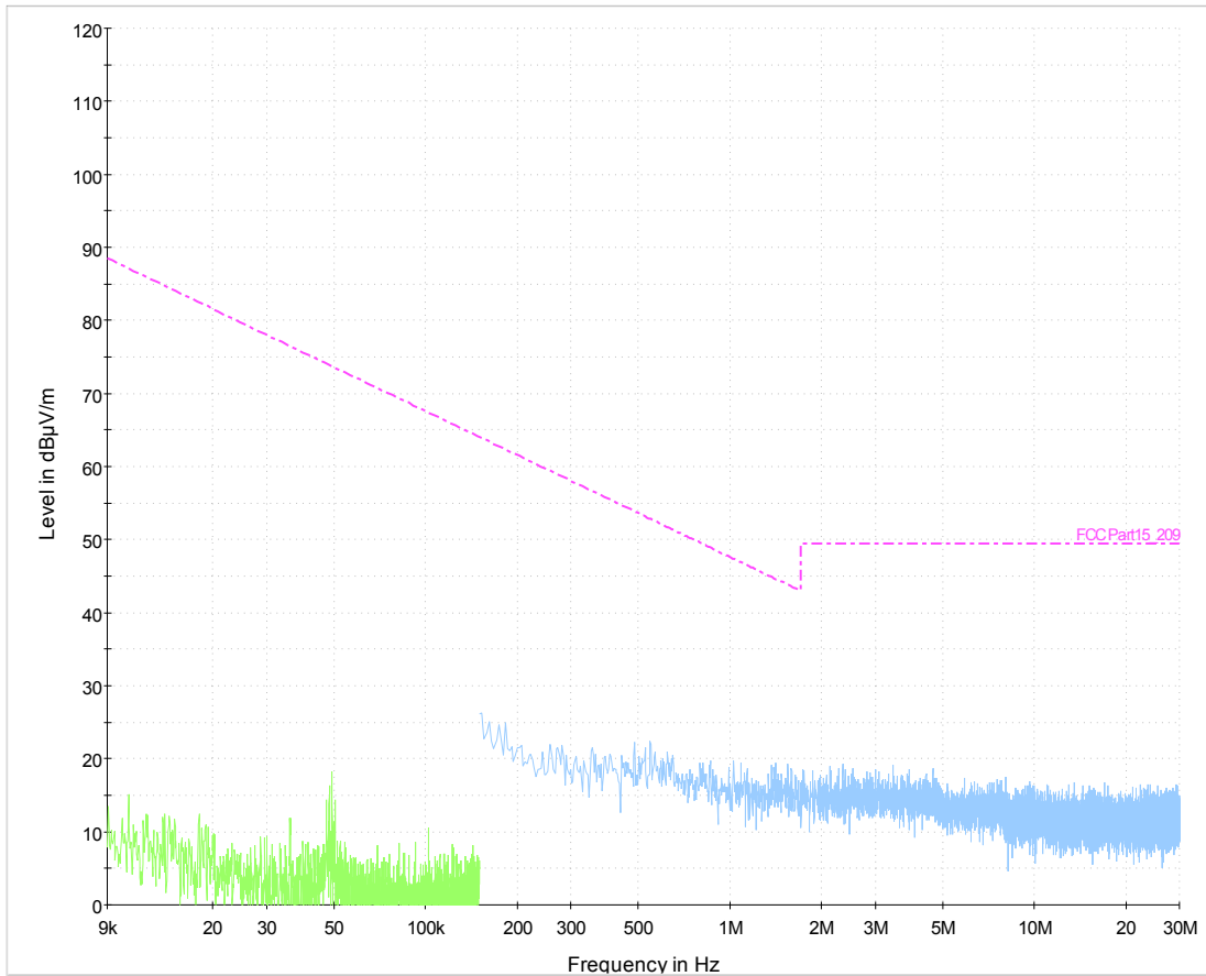
Figure 6-16: Radiated Emissions (9kHz – 30MHz) (middle frequency)
