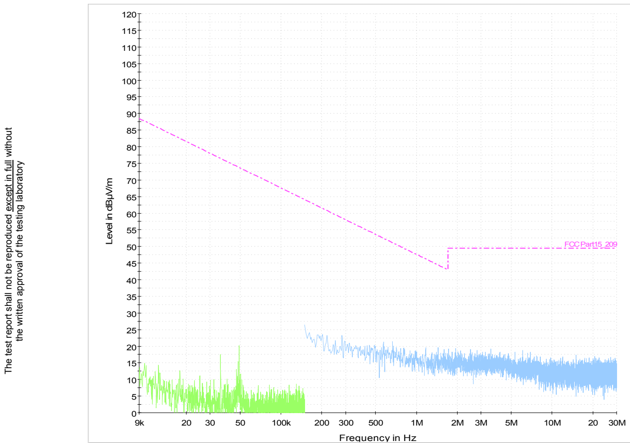
Figure 6-15: Radiated Emissions (9kHz – 30MHz) (bottom frequency)
