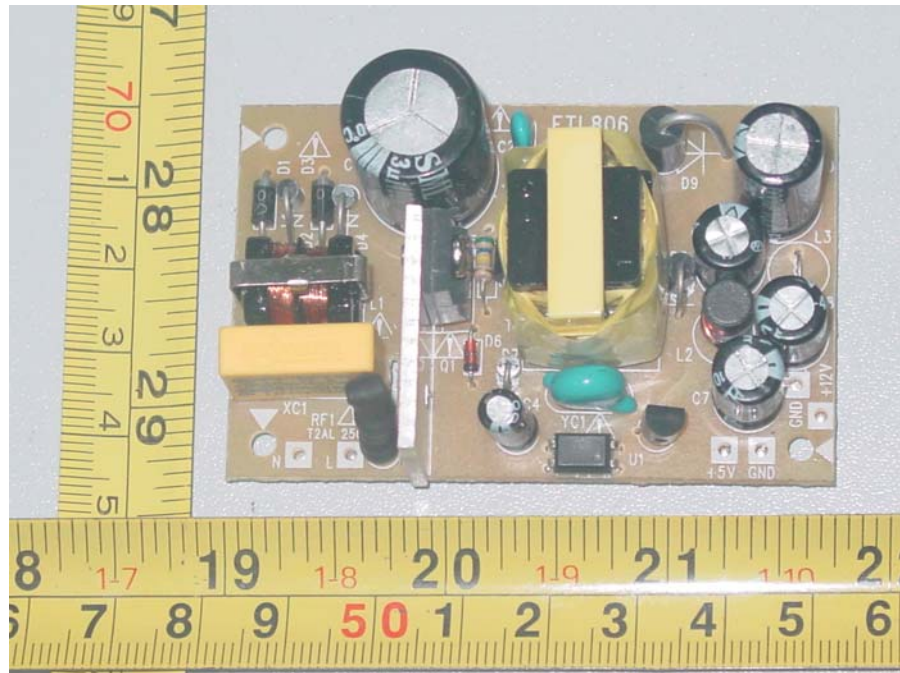
Figure 9 Internal photo of PCB
