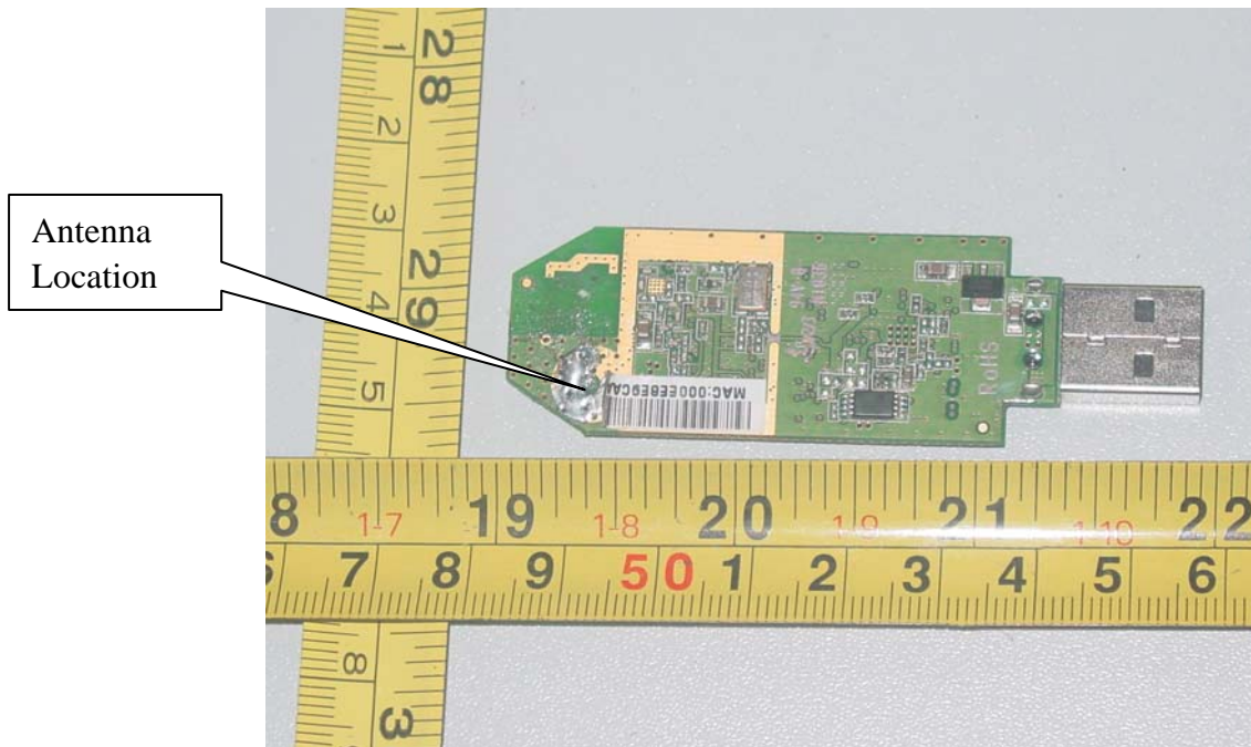
Figure 7 Internal photo of PCB
