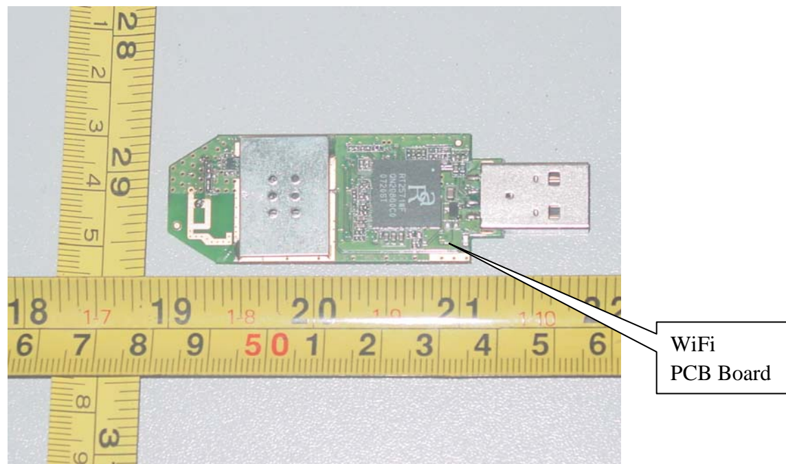
Figure 8 Internal photo of PCB
