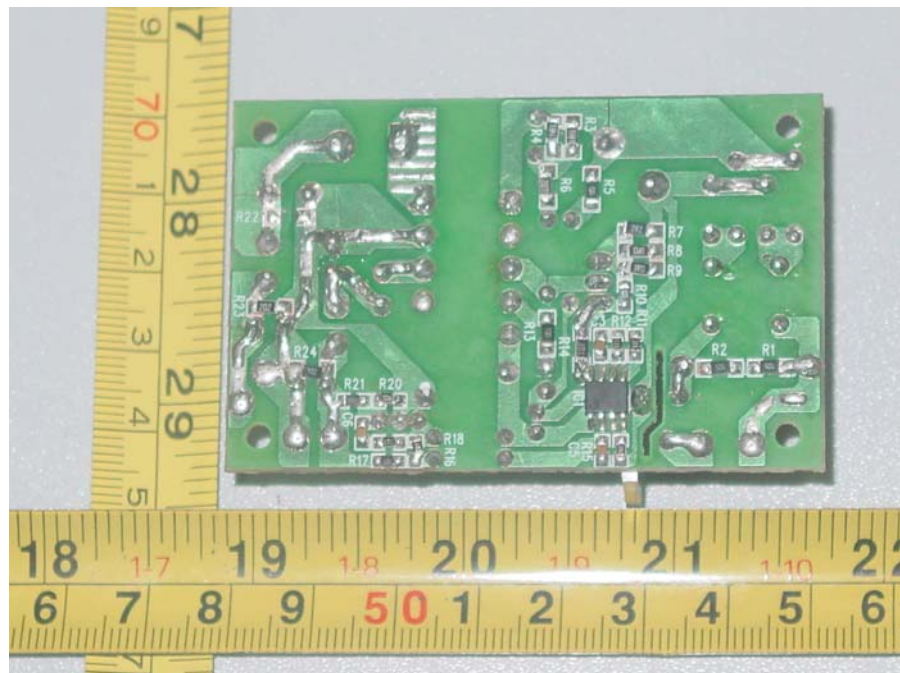
Figure 10 Internal photo of PCB
