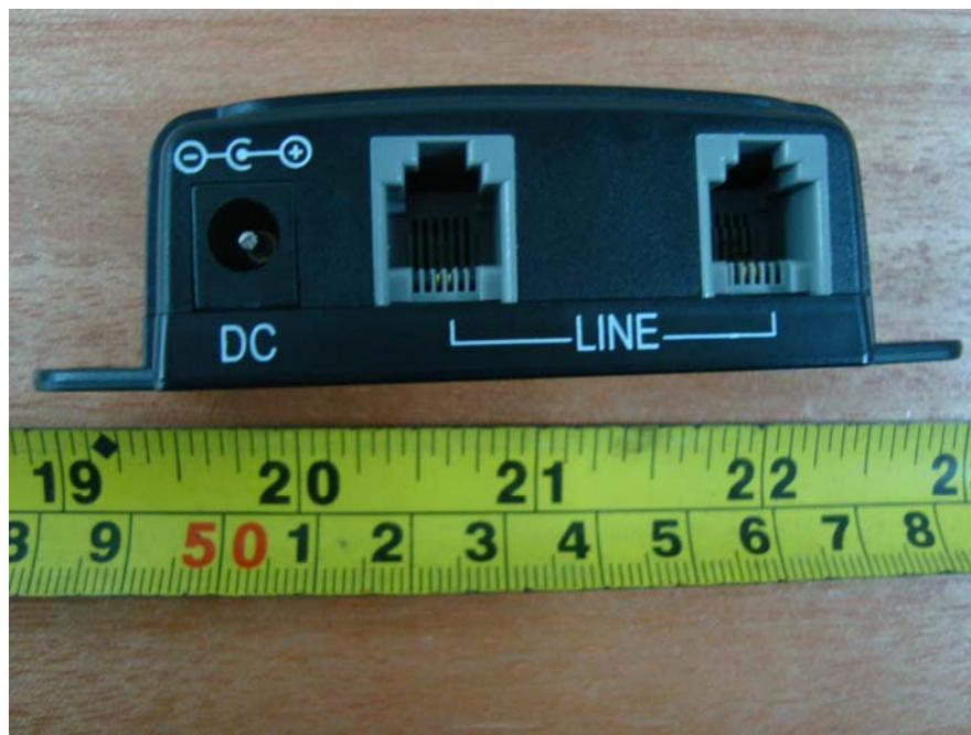
EUT – Connector Box Phone Port View
