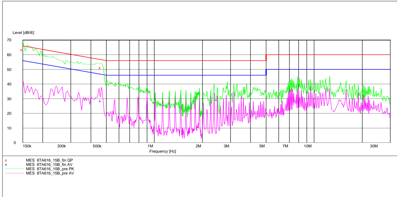
Figure B.3 Conducted Emission
