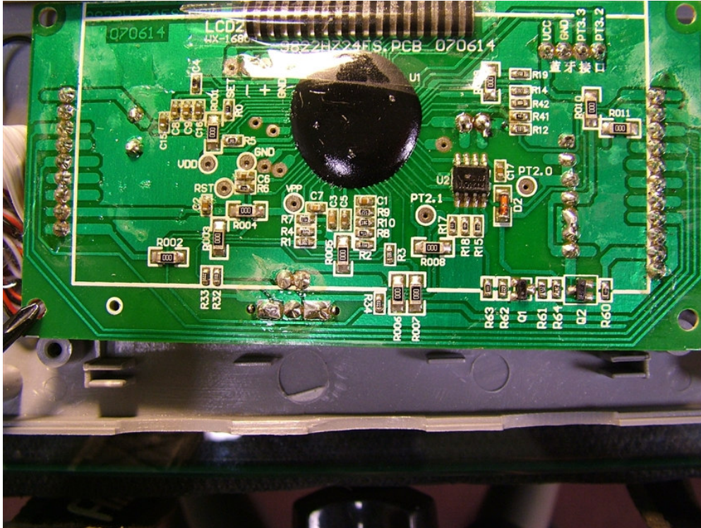
Main processor board
