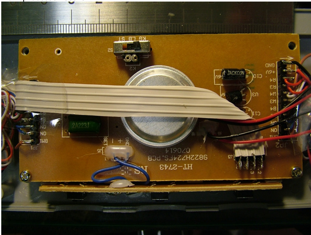
Buzzer and reverse of processor board
