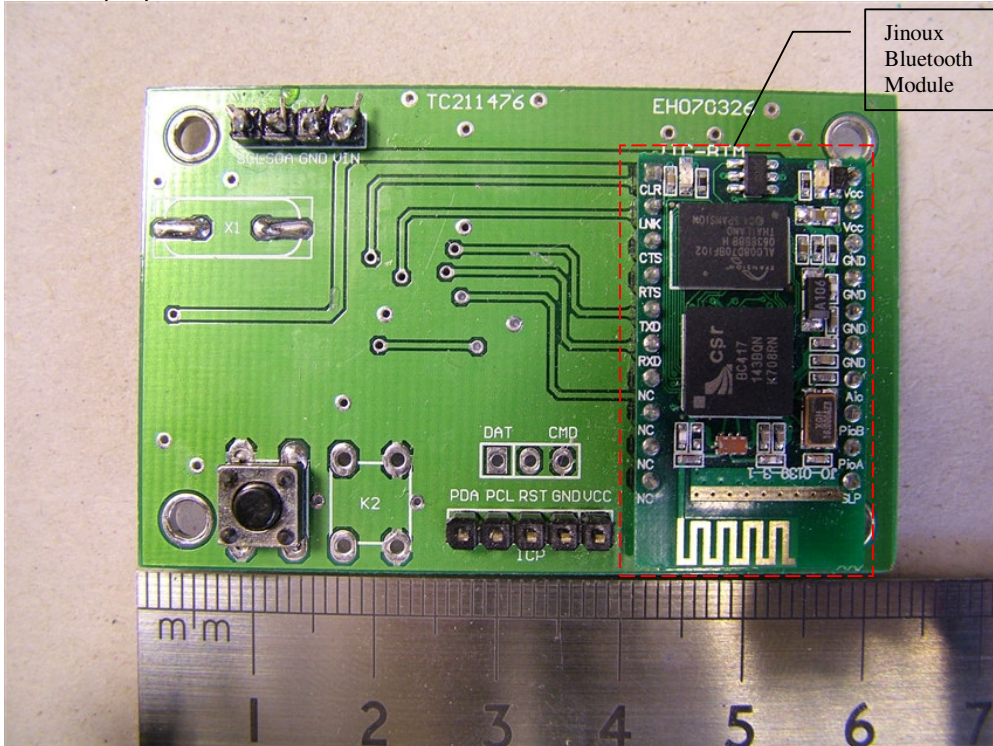
Bluetooth interface board
