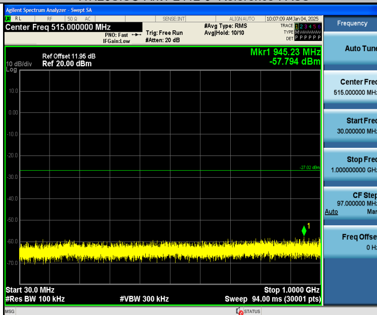
11N20SISO-Ant1-2412-30~1000-PASS
