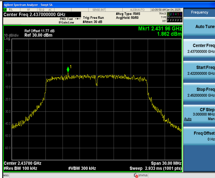
11N20SISO-Ant1-2437-0~Reference-PASS
