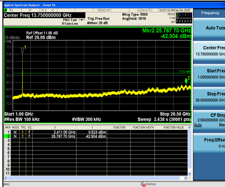
11N20SISO-Ant1-2412-1000~26500-PASS
